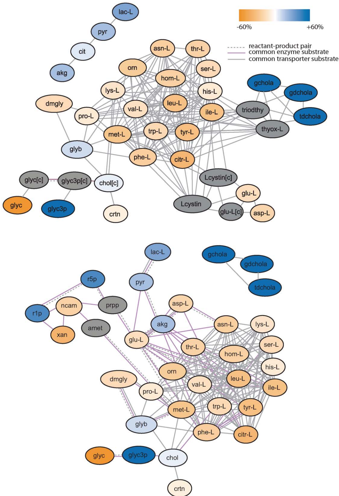
Figure 2. Active Module Groups from the NGT-EMRN and NGT-CMRN. Panels (a) and (b) correspond to NGT-EMRN and NGT-CMRN, respectively. Nodes in the AMG correspond to metabolites in chemical reactions and edges are drawn between reactant-product pairs or shared substrates of enzymes/transporters. A gradient from gold to blue was used to denote reduced percentage change in metabolite abundance after glucose challenge. For clarity, changes were truncated at \pm 60\% . Unmeasured nodes are shown in grey. Edges corresponding to different types of functional links between metabolites are indicated. Cellular locations for metabolites in (a) are assumed to be extracellular unless denoted by [c] for cytoplasmic. Likewise, cellular locations in (b) are assumed to be cytoplasmic unless denoted by [e] for extracellular. The lac-pyr-cit-akg group of metabolites in (a) is connected to the remainder of the set via metabolites with relative frequencies < 0.20 across solutions; the same is true of the bile salts cluster in (b). doi:10.1371/journal.pcbi.1000692.g002
