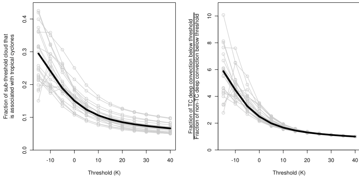
Figure 2. The left panel shows the fraction of annually averaged sub-threshold cloud in the tropics (30° S to 30° N) that is associated with tropical cyclones. The right panel shows the fraction of TC deep-convective cloud that is below the threshold divided by the fraction of non-TC deep-convective cloud that is below the threshold.
