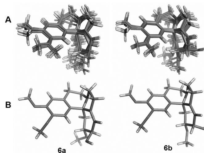
Figure 4. (A) Molecular Dynamics search of conformers (B) optimized geometries for both isomers 6a and 6b .
