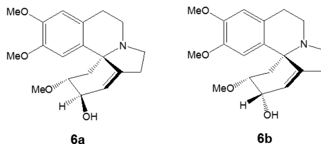
Figure 3. Two alternative structures for epierythratidine 6a and 6b
