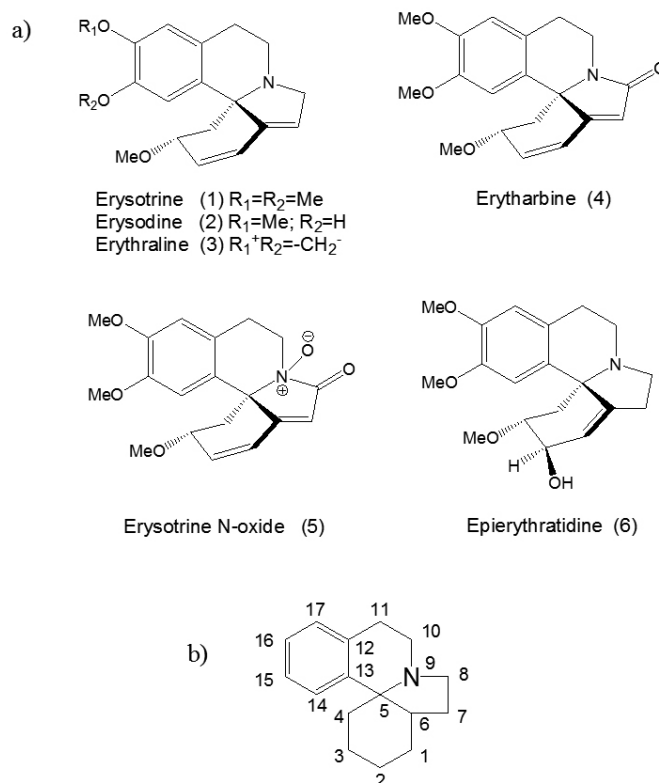
Figure 1. (a) Structures of the alkaloids isolated from seed the Erythrina fusca Lour.
