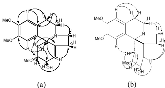
Figure 2. (a) HMBC correlations and (b) NOESY correlations for epierythratidine ( 6 ).
