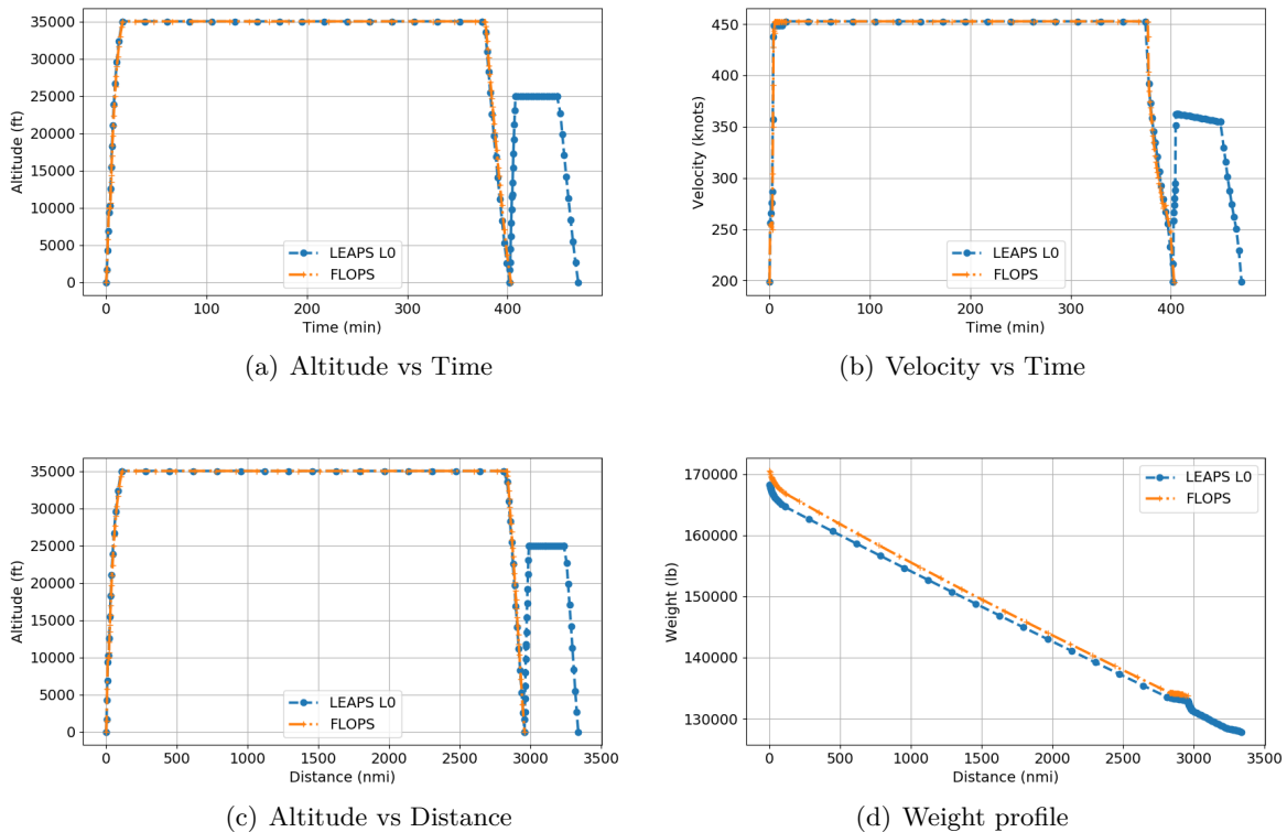
Figure 3: Boeing 737-800 like vehicle mission comparison. LEAPS bounded to match FLOPS trajectory.
