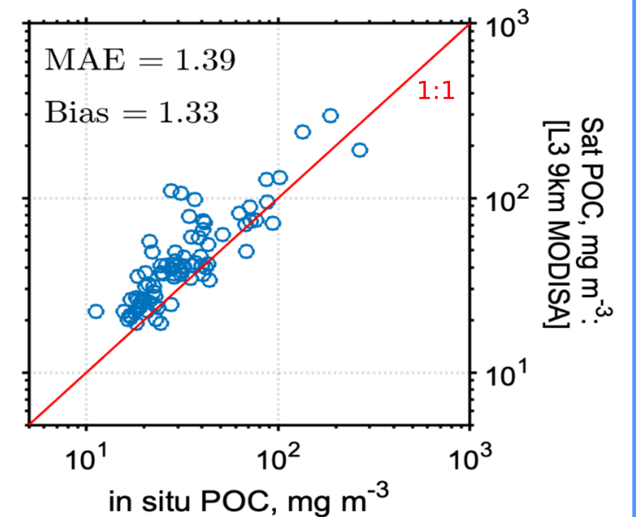
Fig.2. Contemporaneous MODISA L3 9km POC vs. in situ surface POC for the three oceanographic campaigns depicted in Fig. 1. See Fig.1 caption for the definition of multiplicative MAE and bias.
