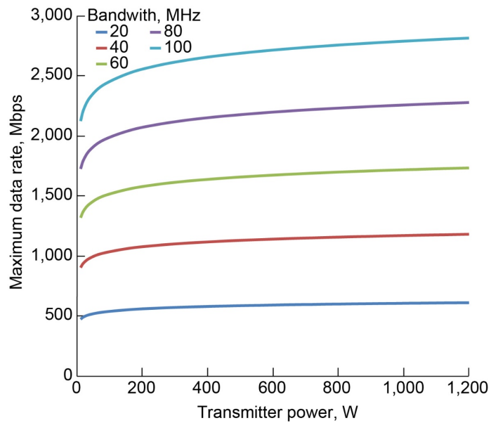
Figure 22.—Transmission power and data rate for lunar surface-to-surface (11.1 km) transmission bandwidths.
