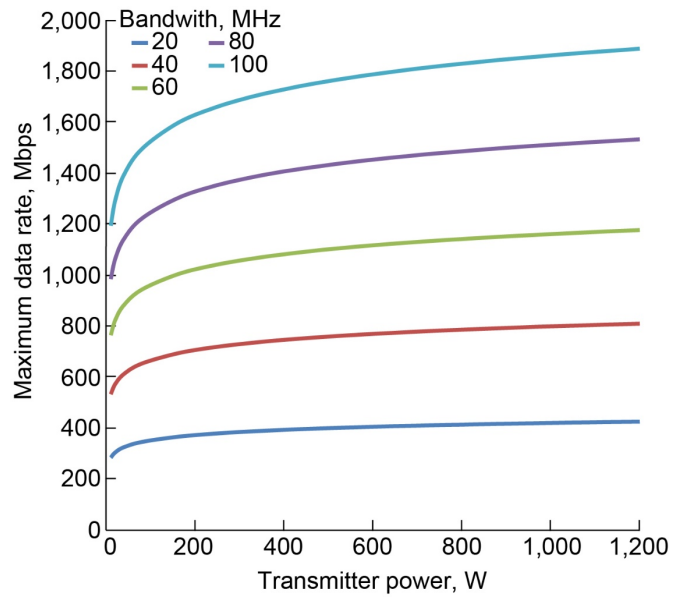
Figure 21.—Transmission power and data rate for lunar surface-to-orbit (6,500 km) transmission bandwidths.
