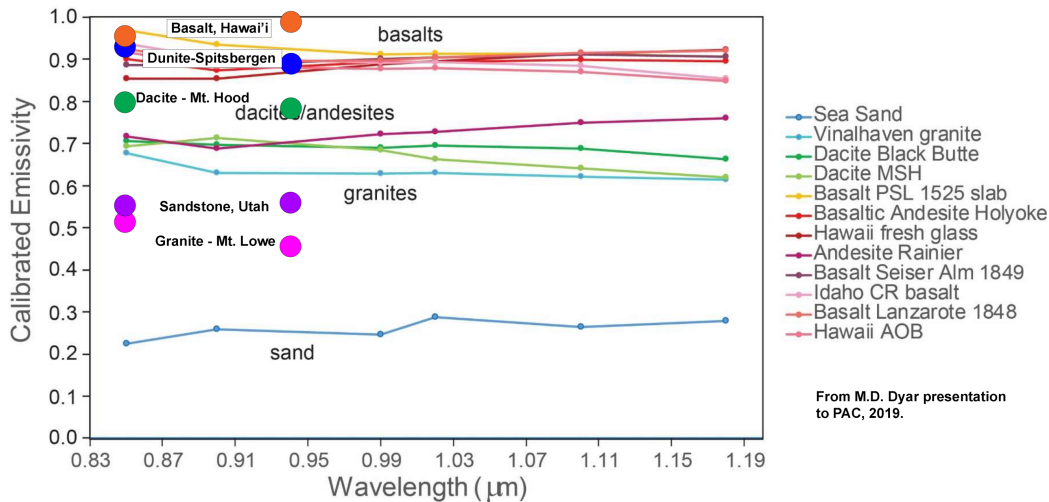
Figure 3. Rock emissivities \epsilon calculated from reflectances r at ~470°C, large filled circles colored as in Fig. 2. Lines and small circles are measured \epsilon values [7]. Base image from [7].
