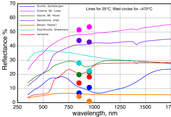
Figure 2. Rock reflectances at 25°C (lines) and at ~470°C (circles), coded to identical colors. To first order, reflectances at high T are similar to those at room T.
