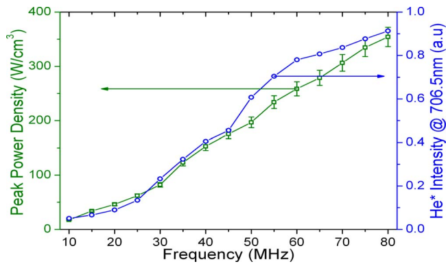
FIG. 2. (Color online) Frequency dependence of the peak dissipated rf power density and the helium 3^3S_1 emission intensity at 706.5 nm.
