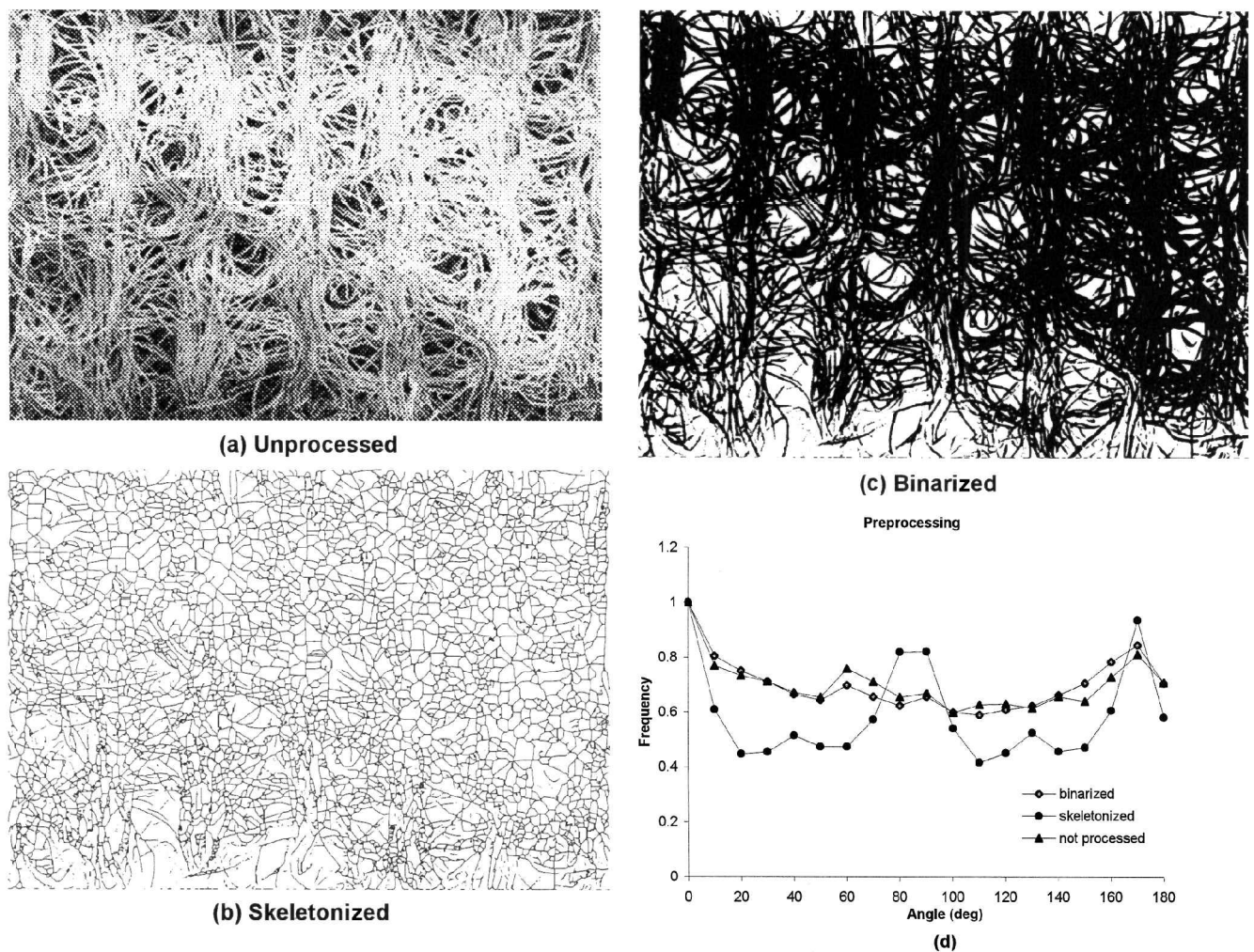
Fig. 10 (a) Sample of the unprocessed image, (b) sample of the skeletonized image, (c) sample of the binarized image and (d) the effect of preprocessing on the result of the fibre orientation distribution
