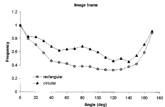
Fig. 9 Effect of the shape of the image frame on the result of the orientation distribution
