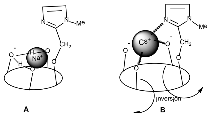
Fig. 1 Ring inversion of O -alkylation intermediate of tetraol 1 and immobilization by metal template.
