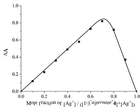
Fig. 5 Job plot for complexation of 1,3-alternate-4 with \text{Ag}^+ ion.
