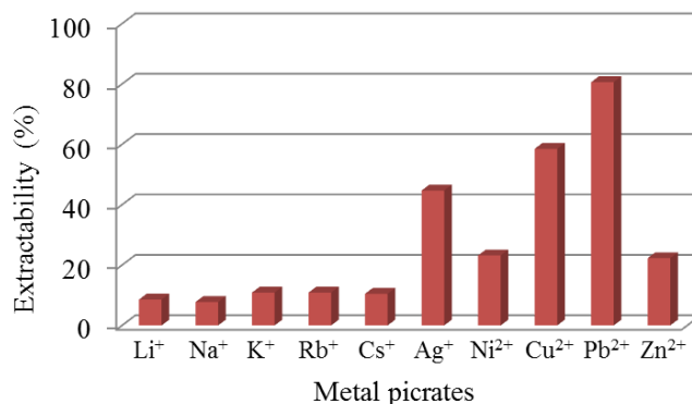
Fig. 4 Extraction percentages of metal picrates with 1,3-alternate-4 ([Host] = 2.5 \times 10^{-4} \text{ M} in \text{CH}_2\text{Cl}_2 , [Guest] = 2.5 \times 10^{-4} \text{ M} in water at 25 °C).
