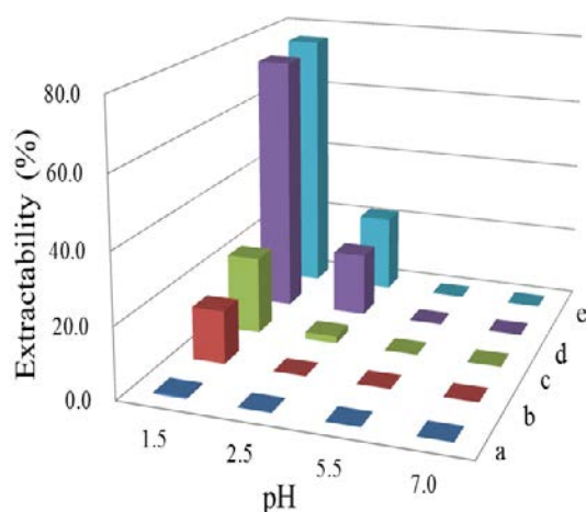
Fig. 8. Extraction percentages of dichromate anion with 1,3- alternate-4 and reference 6 at pH 1.5–7.0 (H 2 O/CH 2 Cl 2 :10/10 (v/v); K 2 Cr 2 O 7 = 1 × 10 -4 M; ligand: (a) reference 6 , 4.0 × 10 -4 M; (b) 1,3- alternate-4 , 0.5 × 10 -4 M; (c) 1,3- alternate-4 , 1.0 × 10 -4 M; (d) 1,3- alternate-4 , 2.0 × 10 -4 M; (e) 1,3- alternate-4 , 4.0 × 10 -4 M, 1 h at 25 °C).
