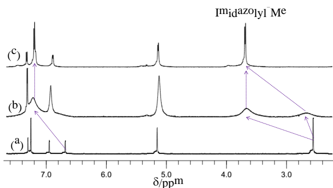
Fig. 6 ^1\text{H} NMR spectral changes of 1,3- alternate-4 ( 8 \times 10^{-3} M) on addition of \text{AgClO}_4 (300 MHz, \text{CDCl}_3:\text{CD}_3\text{CN} = 10 : 1 , [1,3\text{-}i\text{alternate-4}] = 8 \times 10^{-3} M). (a) Free 1,3- alternate-4 ; (b) in the presence of 1.0 equiv. of \text{AgClO}_4 ; (c) in the presence of 2.0 equiv. of \text{AgClO}_4 .
