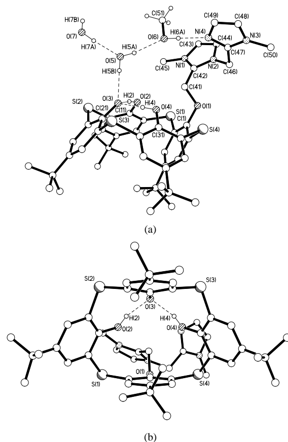
Fig. 2 X-ray structure of compound 3 showing (a) the asymmetric unit including water and methanol of crystallisation, and (b) the upper-rim groups, viewed on to the calix-ring plane. Hydrogen atoms have been omitted for clarity except for those involved in H-bonding or on solvent of crystallisation.
