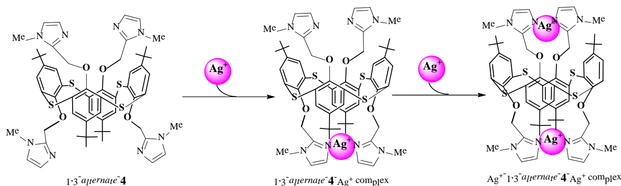
Fig. 7 Binding modes of 1,3- alternate-4 with \text{Ag}^+ .
