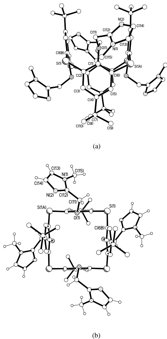
Fig. 3 X-ray structure of compound 1,3-alternate-4 showing (a) the side view (b) the upper-rim groups, viewed on to the calix-ring plane. Hydrogen atoms have been omitted for clarity in (a).
