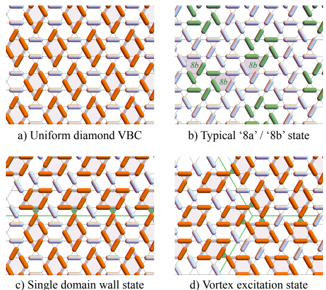
FIG. 4. (a) Uniform diamond VBC state. (b) State with finite density of ‘8b’ processes (2-colored loops). (c) A domain wall separates two different diamond VBC domains. (d) A vortex excitation corresponds to the intersection of three domain-walls. The shaded triangles in (c-d) are the sources of the energy cost of the walls.
