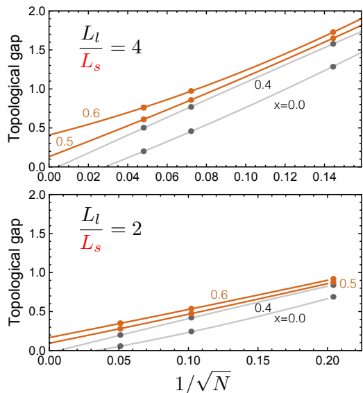
FIG. 8. Evolution of the topological gap as a function of 1/\sqrt{N} , for different fixed ratios of L_\ell/L_s = 4 (top) and 2 (bottom) and various x in the QSL region (gray) and the diamond VBC region (orange).
