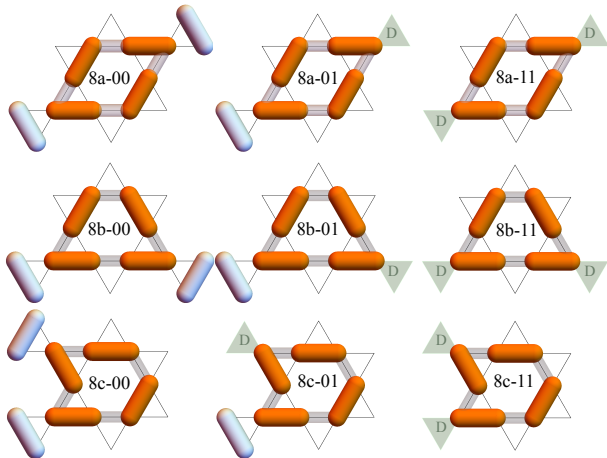
FIG. 2. The most relevant, loop-8 tunneling processes of the microscopic RVB model. Different rows give the three topologically different loops, and different columns designate the dependence of the amplitudes on the possible presence of extra defect triangles nearby.
