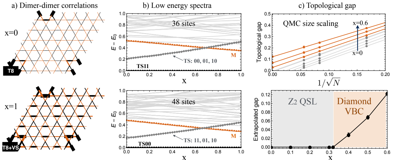
FIG. 3. Numerical results for the minimal model \mathcal{H}_m(x) of Eq. (2). (a) Connected dimer-dimer correlations in the ground state of the 108-site cluster for the ‘T8’ ( x=0 ) and the ‘T8+VS’ ( x=1 ) model. The thick bond on the lower left corner is the reference bond. Positive (negative) correlations are shown by black (red) color. (b) Low-energy spectra as a function of x measured from the ground state energy E_0 and in units of t_6 = 0.127J . The lowest energy states of the four topological sectors are denoted by ‘TS00’, ‘TS01’, ‘TS10’ and ‘TS11’. The level indicated by ‘M’ is the lowest state with momentum at the middle of the Brillouin-zone edge. (c) Topological gap (in units of t_6 = 0.127J ) as calculated from Green’s function Monte Carlo up to 324 sites for various control parameters x . The gap scales well as 1/\sqrt{N} . The lower panel shows the extrapolated value at the thermodynamic limit. The geometry of the clusters is discussed in App. A.
