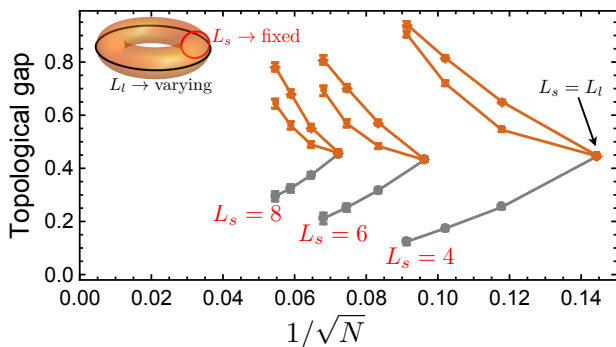
FIG. 7. Topological gap (in units of t_6 = 0.127J ) extracted from GFMC for the ‘T8+VS’ model on tori with L_s \times L_\ell unit cells. There are three sets of data with L_s fixed and L_\ell varying: L_s = 4 (with L_\ell = 4, 6, 8, 10 ), L_s = 6 (with L_\ell = 6, 8, 10, 12 ), and L_s = 8 (with L_\ell = 8, 10, 12, 14 ), see App. A for the specific cluster geometries.
