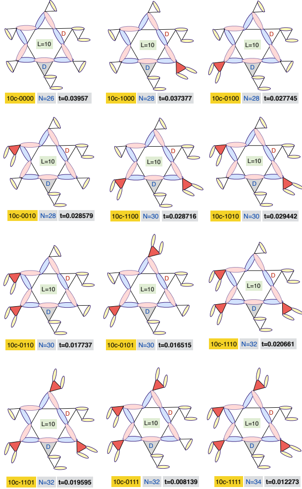
Loop-10, level R2, type 10c
