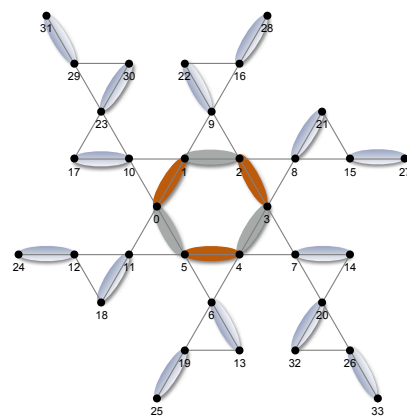
FIG. 9. The 34-site cluster used to extract the parameters t_6 = 0.127J and V_6 = 0.073J given in the main text.
