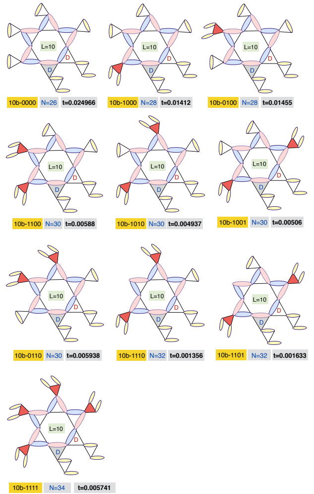
FIG. 12. Heisenberg clusters used to extract the tunneling amplitudes of the type ‘10b’ processes.
