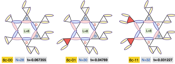
FIG. 10. Heisenberg clusters used to extract the tunneling amplitudes of the type ‘8a’, ‘8b’ and ‘8c’ processes.
