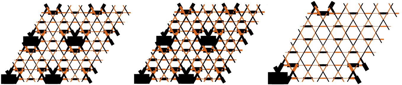
FIG. 6. Dimer-dimer correlations for the ‘R2+E’ model with loop-ten processes excluded on the 48-site cluster (left), the full ‘R2+E’ model on the 48-site cluster (middle), and the full ‘R2+E’ model on the 108-site cluster (right). The thick black segment at the bottom-left corner denotes the reference dimer. The 48-site cluster is periodically repeated four times for convenience. Black (orange) color indicates positive (negative) correlation values. The thickness of each dimer scales with the magnitude of the correlation. The diamond VBC order can be seen by the pattern of the positive correlations (black segments).
