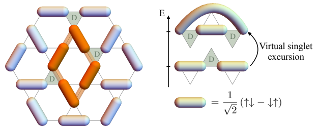
FIG. 1. A dimer covering of the kagome lattice, where each dimer represents a spin singlet between NN spins. Tunneling processes shift the dimers around closed loops (orange). Such processes are mediated by longer-range singlets that are virtually excited around empty, or ‘defect’ triangles (D). The ensuing amplitude depends on the particular dimer environment outside the loop. 32,58
