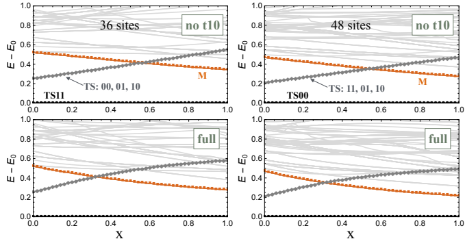
FIG. 5. Spectrum of \mathcal{H}_m(x) with loop-6 (top), and loop-6 plus loop-10 (bottom) processes added.
