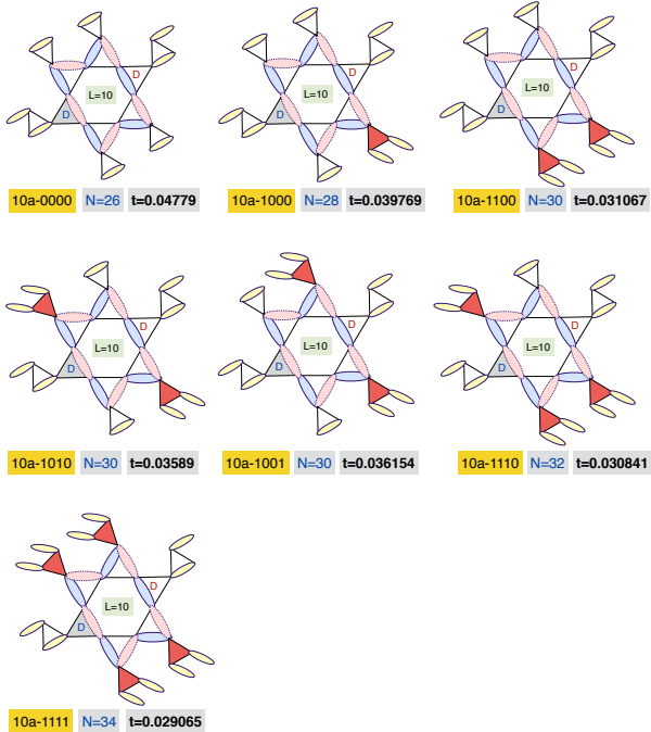
FIG. 11. Heisenberg clusters used to extract the tunneling amplitudes of the type ‘10a’ processes.
