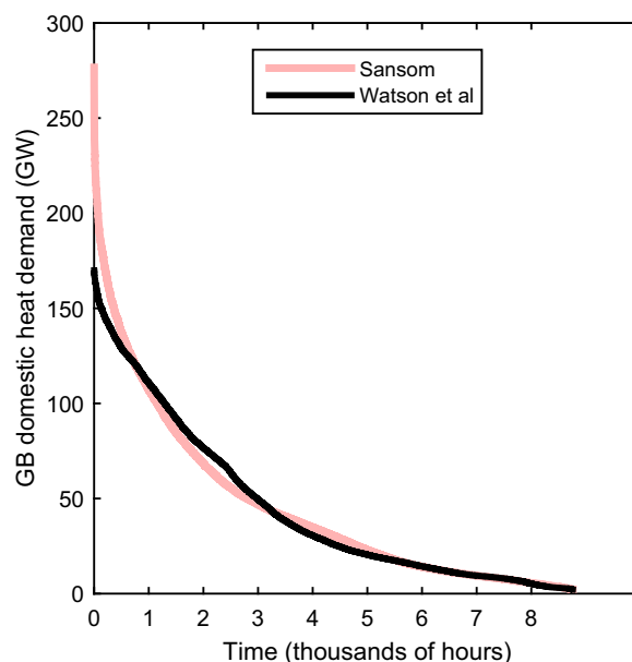
Fig. 12. Load duration curve for GB domestic heat demand for 2010, produced here and to according to Sansom.
