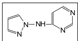
Figure 40. Structure of 6-aminopyrazolopyrimidine.
