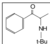
Figure 22. Structure of bupropion.
