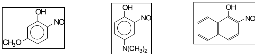
Figure 13. Structure of 5-methoxy- and 4-(dimethylamino)-2-nitrosophenol and 1-nitroso- \alpha -naphthol.
