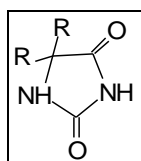
Figure 32. Structure of 5,5-disubstituted hydantoins.
