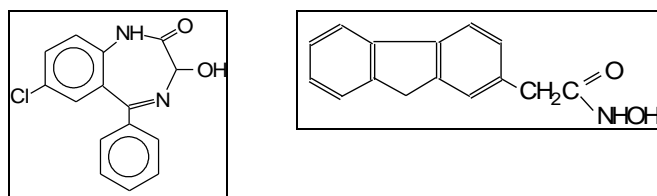
Figure 9. Structures of oxazepam and N-hydroxy-2-fluorenylacetylacetamide.
