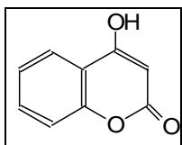
Figure 23. Structure of 4-hydroxycoumarin.
