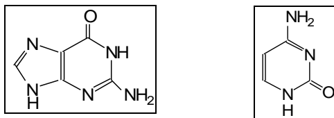
Figure 33. Structure of guanine and cytosine.
