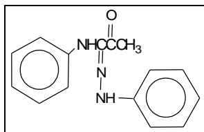
Figure 5. Structure of 2,3-dioxobutanilide-2-phenylhydrazone.
