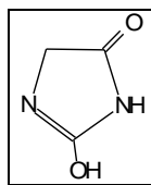
Figure 47. Structure of the preferred enolic form of hydantoin.
