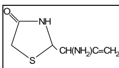
Figure 4. Structure of 2-(allylamino)thiazolin-4-one.
