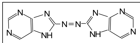
Figure 38. Structure of 8,8'-azopurine.
