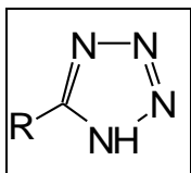
Figure 39. Structure of 5R-tetrazols.
