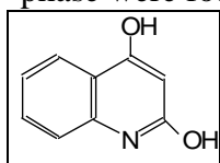
Figure 25. Structure of 2,4-dihydroxyquinoline.
