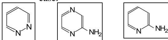
Figure 31. Structures of pyridazine, aminopyrazine and aminopyridine.
