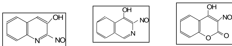
Figure 17. Structures of o -hydroxynitroso derivatives of quinoline, isoquinoline and coumarin.
