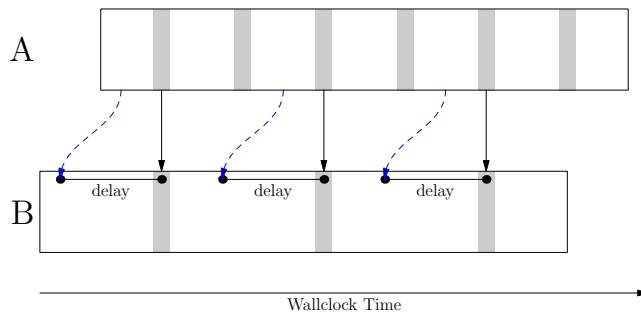
Figure 2.4: This figure illustrates how MUSIC can allow one application (A) to execute ahead of another (B) when transferring continuous data. The receiver (B) has specified a delay on the input port which means that the value to be delivered at each tick (gray areas) corresponds to a simulated time in A (blue arrows) which has already happened.
