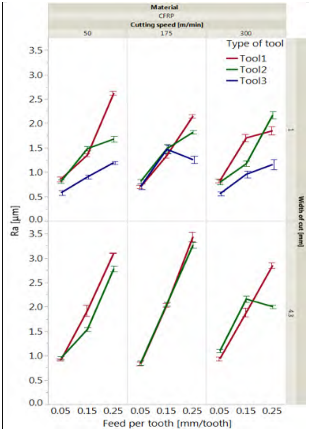
Figure 3.23 Ra on the CFRP plaque in function of different cutting parameters v , ae and ft giving by \pm SEM
