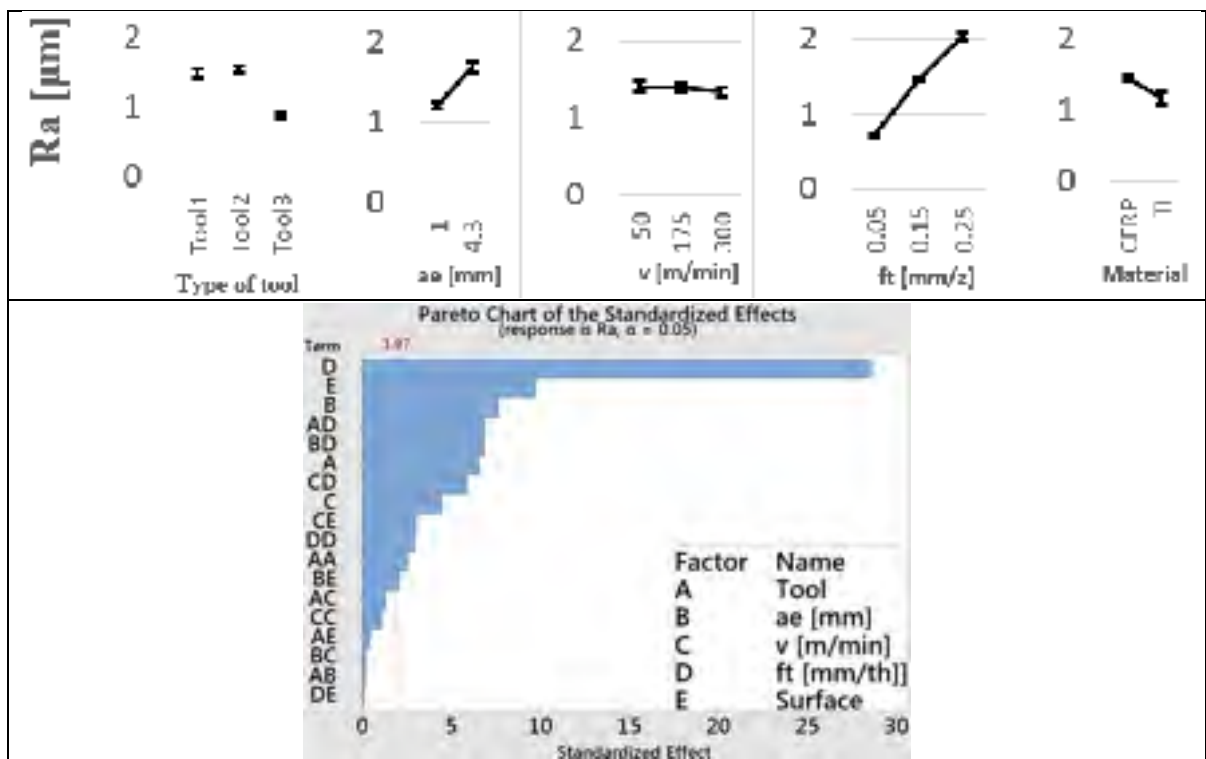
Figure 3.22 Main Effect plot of Ra in function to different parameters giving by \pm SEM and Ra Pareto chart of the most significant factor
