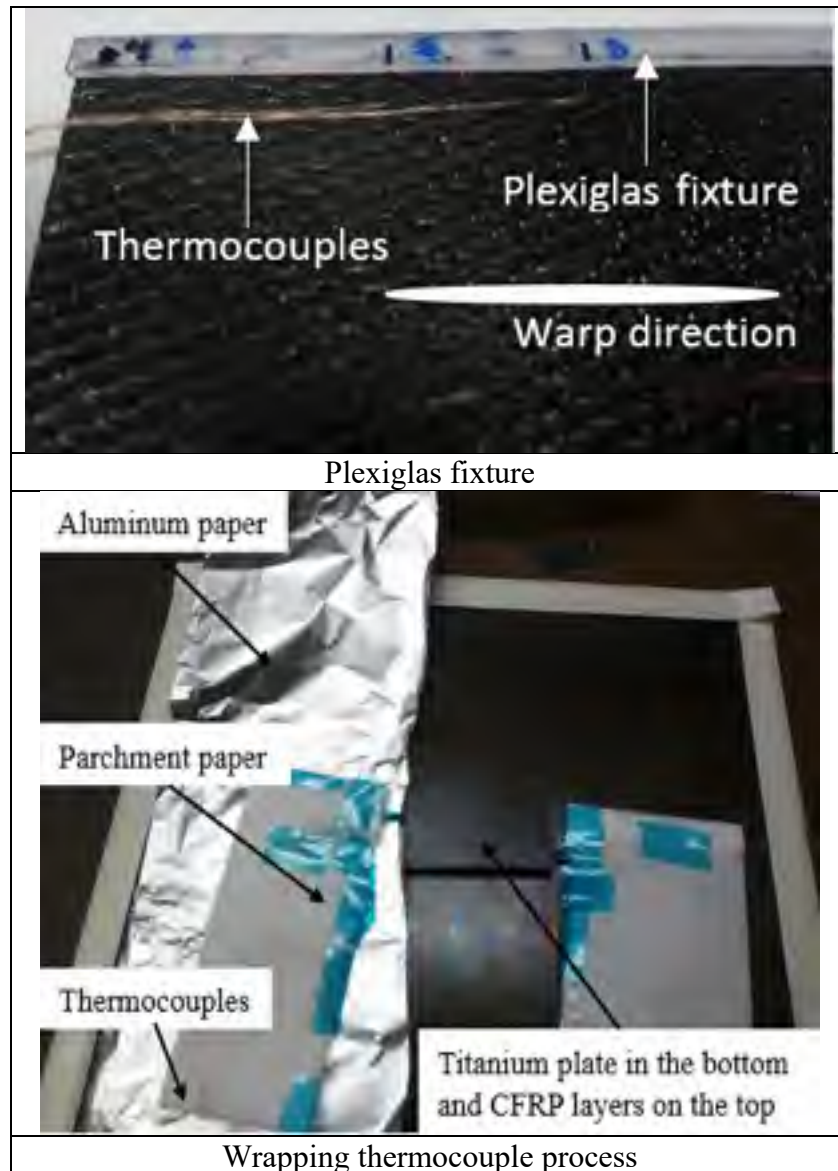
Figure 2.10 Thermocouples setup process
