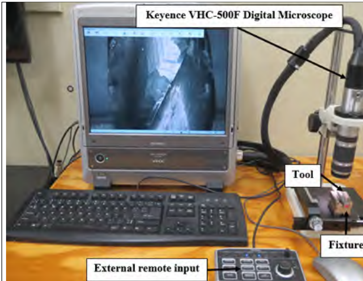
Figure 2.19 Setup to measure tool wear
