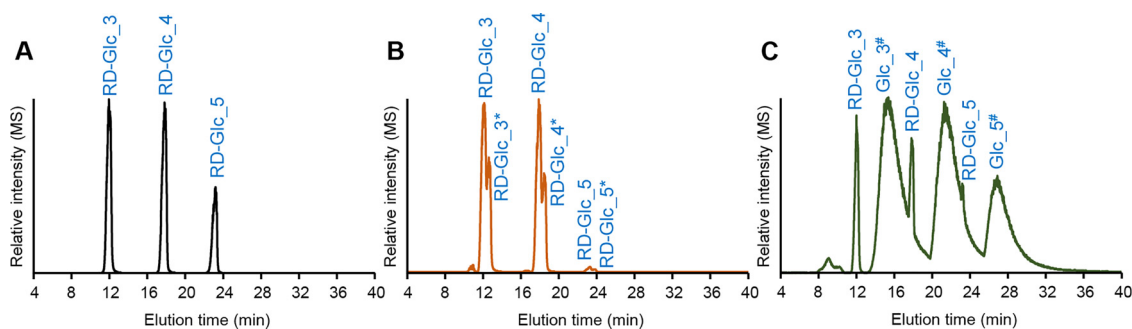
Fig. 4. HILIC extracted ion chromatograms of NaBD 4 -reduced non-, C4- and C1-oxidised cello-oligosaccharides. (A) Reduced non-oxidised cello-oligosaccharides: RD-Glc_3, m/z 506.3; RD-Glc_4, m/z 668.3; RD-Glc_5, m/z 830.3; (B) Both reduced non- and C4-oxidised cello-oligosaccharides: RD-Glc_3–5 m/z see explanation panel A; RD-Glc_3*, m/z 507.2; RD-Glc_4*, m/z 669.3; RD-Glc_5*, m/z 831.3; (C) Reduced non- and C1-oxidised cello-oligosaccharides: RD-Glc_3–5, m/z see explanation panel A; Glc_3#, m/z 519.2; Glc_4#, m/z 681.3; Glc_5#, m/z 843.3.
