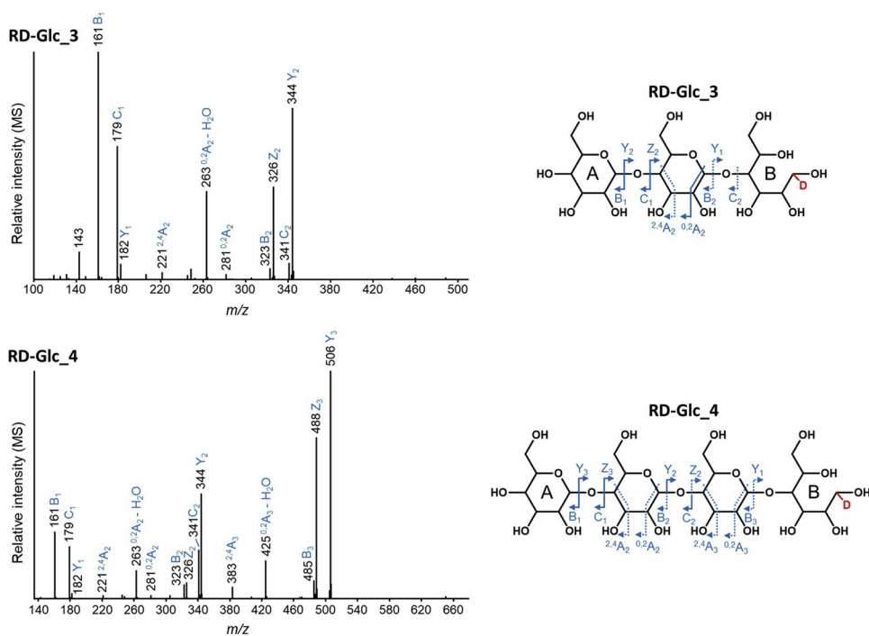
Fig. 5. Negative ion mode CID-MS/MS spectra of reduced non-oxidised cello-oligosaccharides DP3 (RD-Glc_3, m/z 506.3) and DP4 (RD-Glc_4, m/z 668.3). See Fig. S10 for DP5 (RD-Glc_5, m/z 830.3); average spectra across chromatographic peaks. The fragments are annotated according to Domon and Costello (1988). Blue solid arrows indicate the most abundant fragments, while dashed arrows indicate fragments with relatively lower intensity. The deuterium ion is indicated in red. A and B ring represent the non-reducing and deuterated alditol end, respectively (For interpretation of the references to colour in this figure legend, the reader is referred to the web version of this article).
