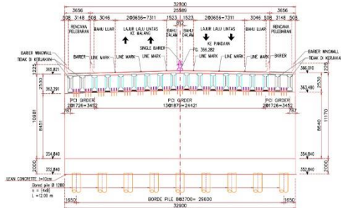
Gambar 4. Potongan Abutment
