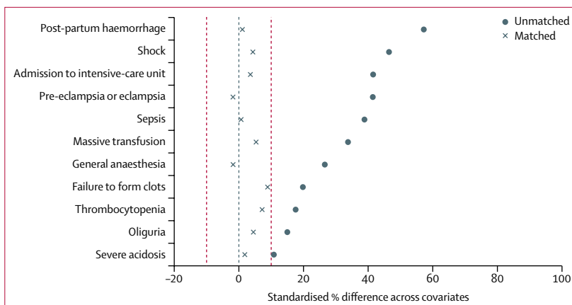
Figure 2: Propensity score matching of cases of severe anaemia with cases without severe anaemia Red dotted lines denote 10% standardised difference between covariates. The appendix details the confounding variables included.
