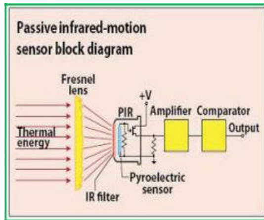
Gambar 5. Blok diagram sensor PIR
