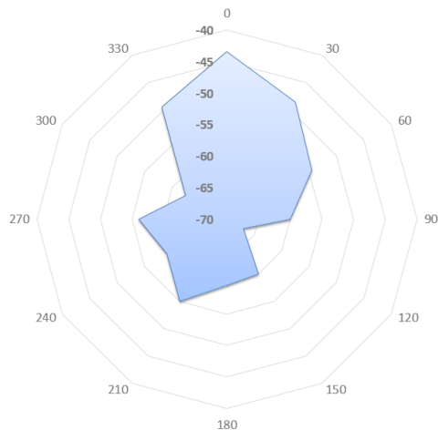
Figure 5: RSSI values received from a directional antenna, depending on the angle of orientation.
