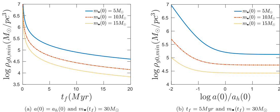
Figure 1: Minimum initial density of the gas ( \rho_{g0,min} ), given in Equation (37), required for a BBH with equal mass BH members so that each member reaches mass 30M_\odot by Bondi accretion inside this gas’ density environment and until time t_f when the gas is completely depleted, assuming a constant mass loss rate of the gas (31). For an exponential gas loss law (32), the time t_{99} needed for 99% depletion is t_{99} = 2.3t_f , for the same values of all other parameters. We also assume in both figures c_s = 5km/s , \sigma = v_c = 6km/ where we denote, respectively, the speed of sound of the gas, the velocity dispersion of the stars and the velocity of the binary with respect to the cluster. We consider three cases, each member having initial mass m_0 = 5M_\odot (blue solid line), 10M_\odot (red dashed-dotted line) or 15M_\odot (yellow dashed line). Left: We assume an initially slightly hard binary with \chi(0) = 1 \Leftrightarrow a(0) = a_h(0) . It is evident that in order for a BH with initial mass \sim (5 - 10)M_\odot to grow up to 30M_\odot within t_f = 5Myr , assuming by this time there is complete gas depletion, would require an initial gas’ density \sim (5 - 15) \cdot 10^4 M_\odot/pc^3 . These minimum density values correspond to the exponential gas loss law with 99% depletion at time t_{99} = 11.5Myr . The density values are half for t_f = 10Myr for both linear and exponential cases. We took into account the hardening of the binary during accretion. Right: We calculate \rho_{g0,min} w.r.t. the initial hardness expressed by the quantity \log \chi^{-1}(0) for t_f = 5Myr in the linear case of gas loss. This time corresponds to t_{99} = 11.5Myr in the case of exponential gas loss. It is evident that soft binaries accrete gas more effectively than very hard ones. A hard binary a(0)/a_h(0) = 0.1 with BH members each of mass (5 - 10)M_\odot requires \rho_{g0,min} = (8 - 50) \cdot 10^4 M_\odot/pc^3 while a soft one a(0)/a_h(0) = 10 requires only (5 - 13) \cdot 10^4 M_\odot/pc^3 . By the time the gas is depleted a soft binary gets hard in case of isotropic accretion as demonstrated below, in Figure 2.
