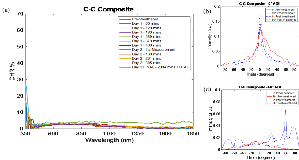
Fig. 6. The (a) reflectance spectrum and BRDF results at (b) 0° and (c) 60° angles of incidence for pre- and post-weathered c-c composite measured during Campaign #2.
