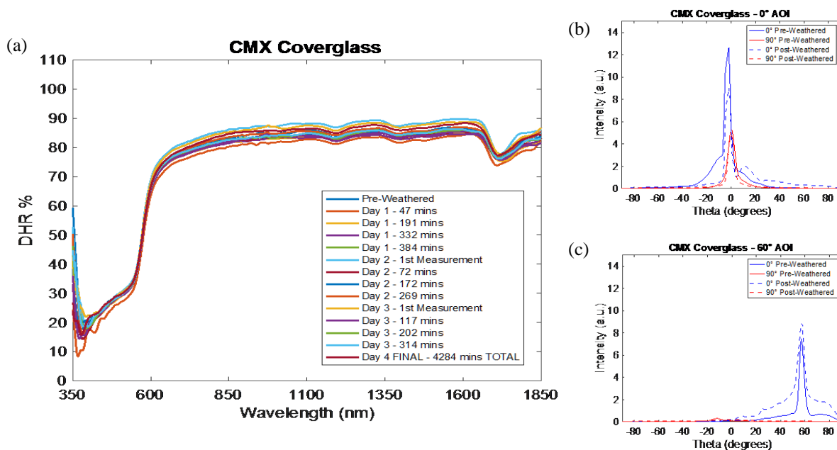
Fig. 4. The (a) reflectance spectrum and BRDF results at (b) 0° and (c) 60° angles of incidence for pre- and post-weathered CMX cover glass measured during Campaign #1.
