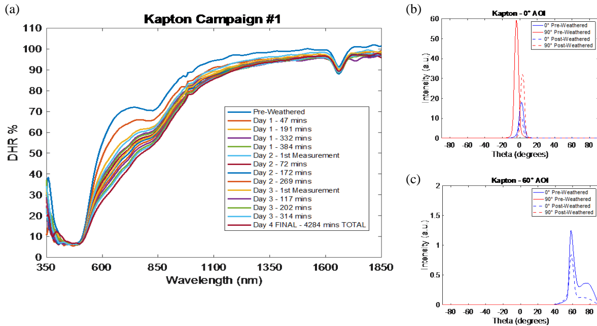
Fig. 9. The (a) reflectance spectrum and BRDF results at (b) 0^\circ and (c) 60^\circ angles of incidence for pre- and post-weathered Kapton measured during Campaign #1.
