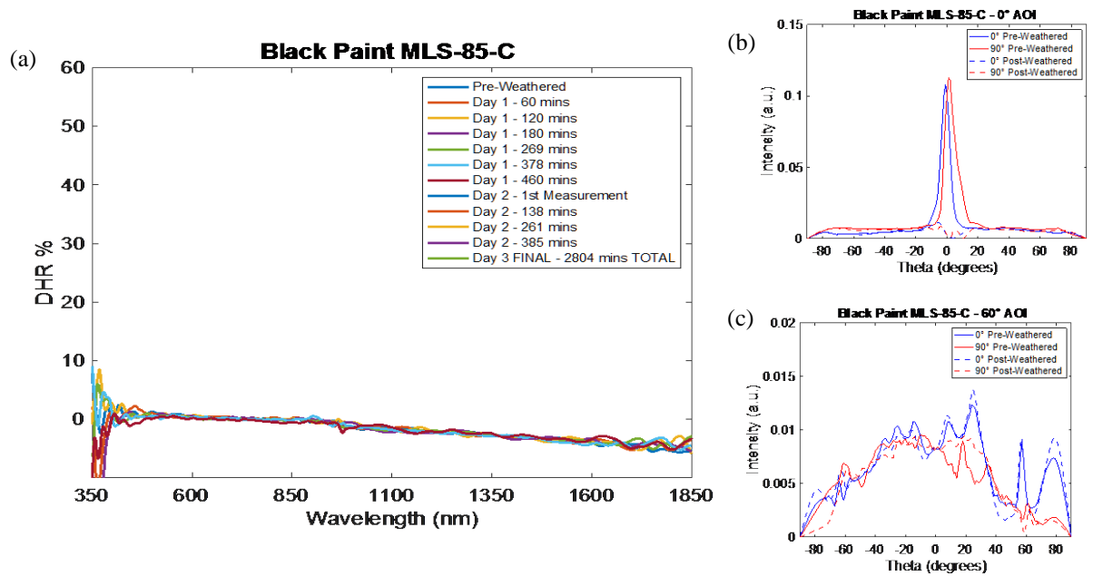
Fig. 8. The (a) reflectance spectrum and BRDF results at (b) 0° and (c) 60° angles of incidence for pre- and post-weathered black paint MLS-85-C measured during Campaign #2.
