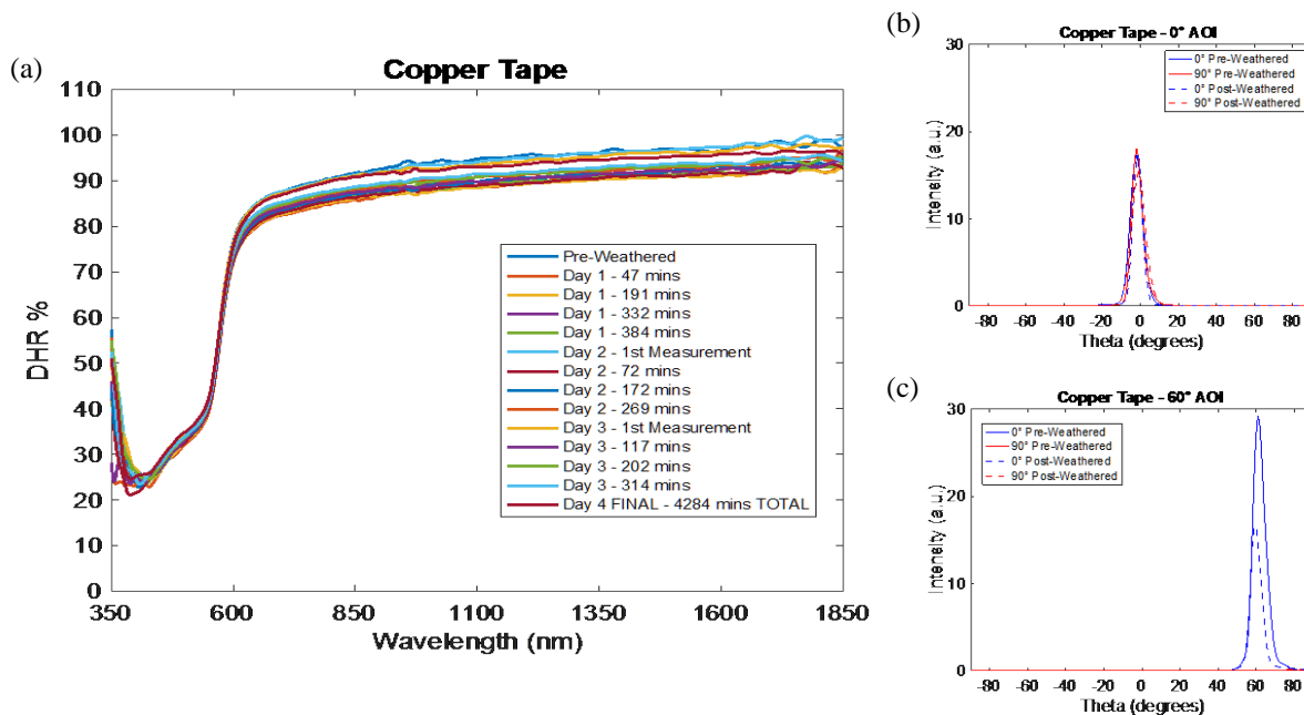
Fig. 5. The (a) reflectance spectrum and BRDF results at (b) 0° and (c) 60° angles of incidence for pre- and post-weathered Cu tape measured during Campaign #1.
