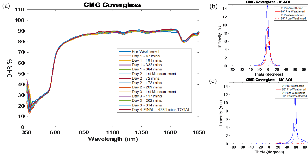
Fig. 3. The (a) reflectance spectrum and BRDF results at (b) 0° and (c) 60° angles of incidence for pre- and post-weathered CMG cover glass measured during Campaign #1.
