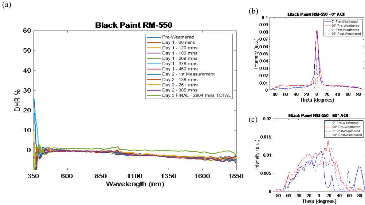
Fig. 7. The (a) reflectance spectrum and BRDF results at (b) 0° and (c) 60° angles of incidence for pre- and post-weathered black paint RM-550 measured during Campaign #2.
