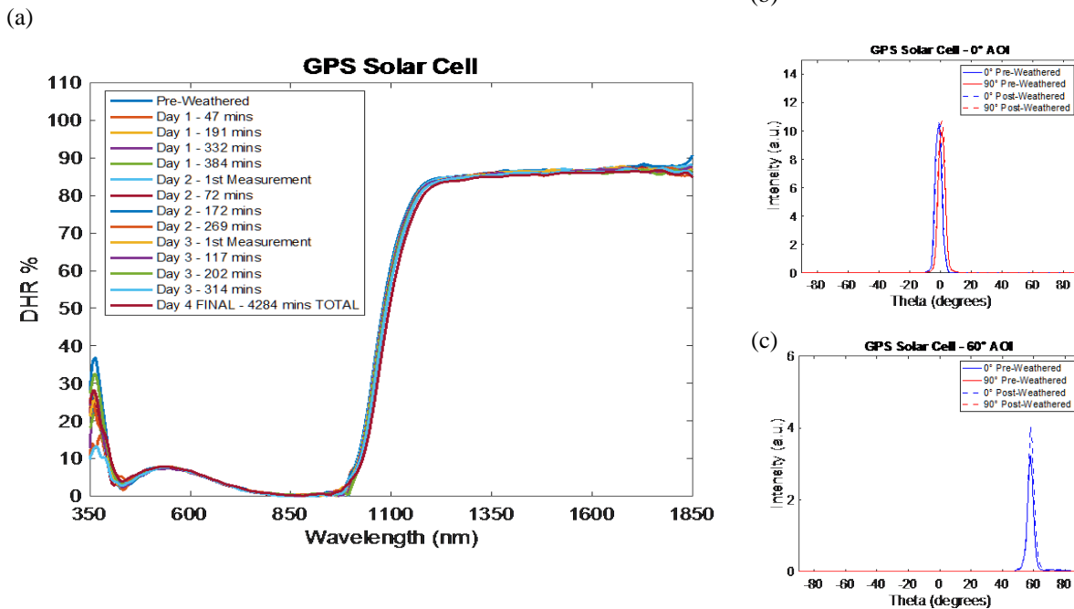
Fig. 2. The (a) reflectance spectrum and BRDF results at (b) 0° and (c) 60° angles of incidence for pre- and post-weathered GPS Solar Cell measured during Campaign #1.
