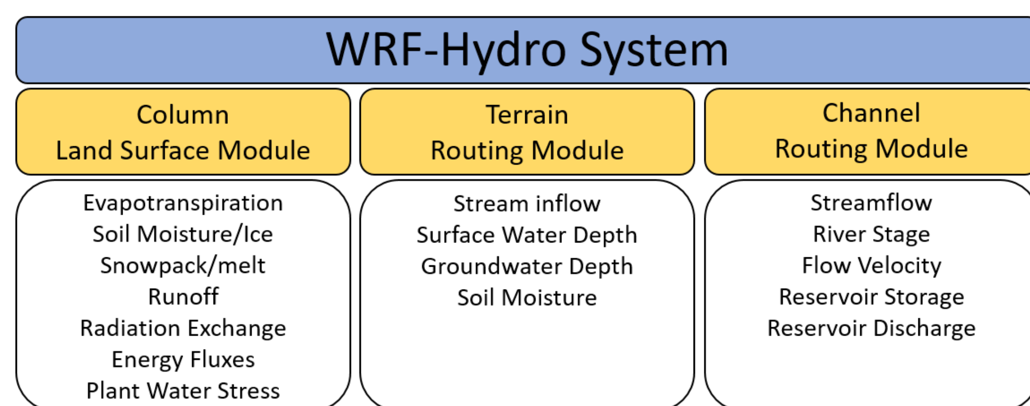
Figure 1. WRF-Hydro modules and output variables (NCAR 2019)
