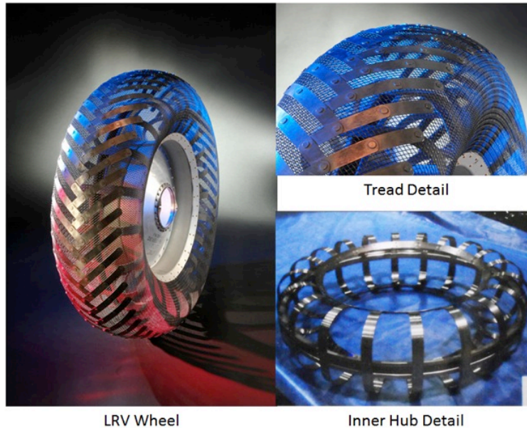
Figure 4.6.—Lunar rover wheel.
