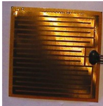
Figure 4.27.—DuPont Kapton Strip Heater.
