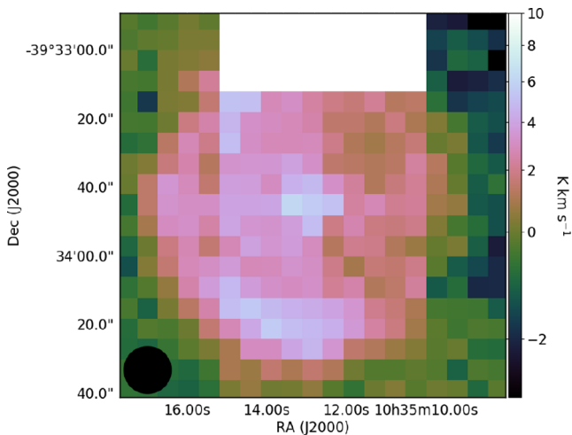
Figure B1. Integrated ^{12}\text{CO}(3-2) HARP observation of U Ant used to carry out CO subtraction on the SCUBA-2 850 \mu\text{m} observation. Filled black circle in the bottom left corner: HARP beam with FWHM of 14 arcsec. The figure is integrated over the velocity range of [-26, 82] \text{km s}^{-1} .
