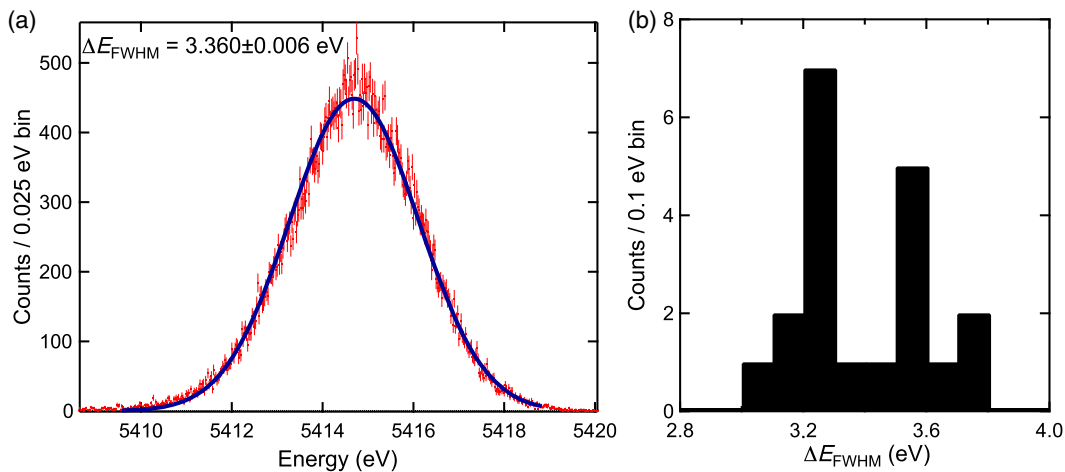
Fig. 9 (a) Co-added spectrum including all 20 pixels in the hydra for monochromatic x-rays taken from Cr-K α1 . A Gaussian fit to the energy histogram gives \Delta E_{\text{FWHM}} = 3.360 \pm 0.006 eV, consistent with the RMS of individual pixels. (b) Histogram of individual energy resolutions for all 20 pixels.
