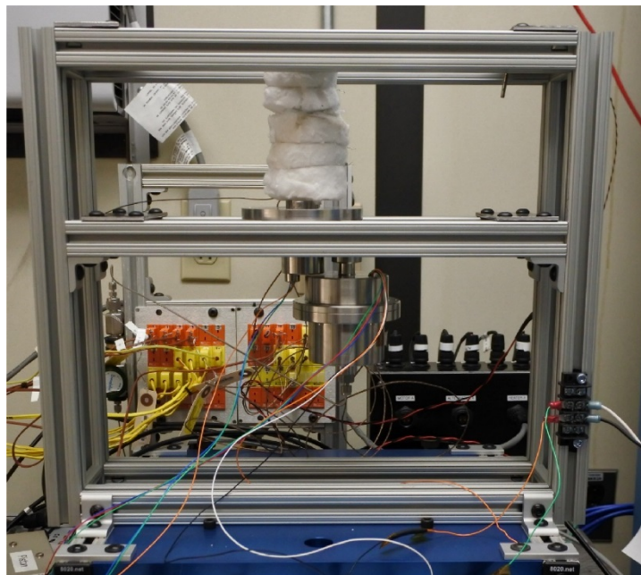
Figure 11.—Extruded aluminum rigid converter mounting structure.
