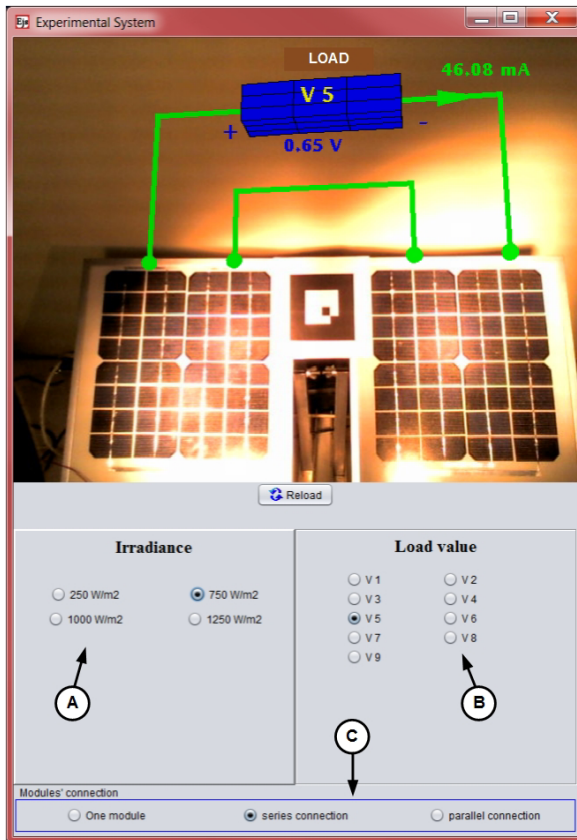
Fig. 2 User interface of the photovoltaic panels remote lab
