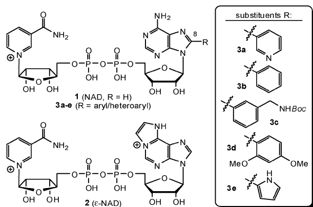
Fig. 1 Chemical structures of natural NAD 1 , 1, N 6 -ethenoadenine dinucleotide 2 , and NAD derivatives 3a–e developed in this study.
