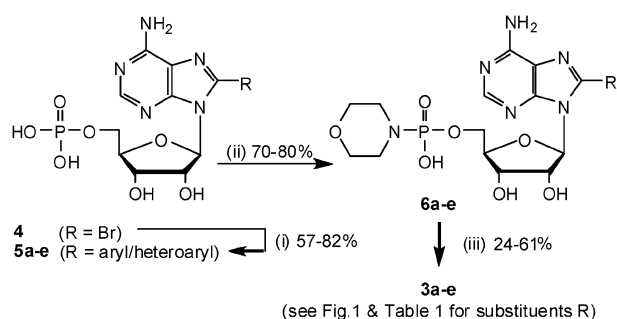
Scheme 1 Reagents and conditions: (i) \text{Na}_2\text{PdCl}_4 , TPPTS, R-B(OH) _2 , \text{K}_2\text{CO}_3 , \text{H}_2\text{O} , \Delta , 1–24 h; (ii) morpholine, dipyridyldisulfide, \text{Ph}_3\text{P} , DMSO, rt, 2 h; (iii) \beta -NMN, dry \text{MgSO}_4 , \text{MnCl}_2 0.2 M in formamide, rt, 24 h.
