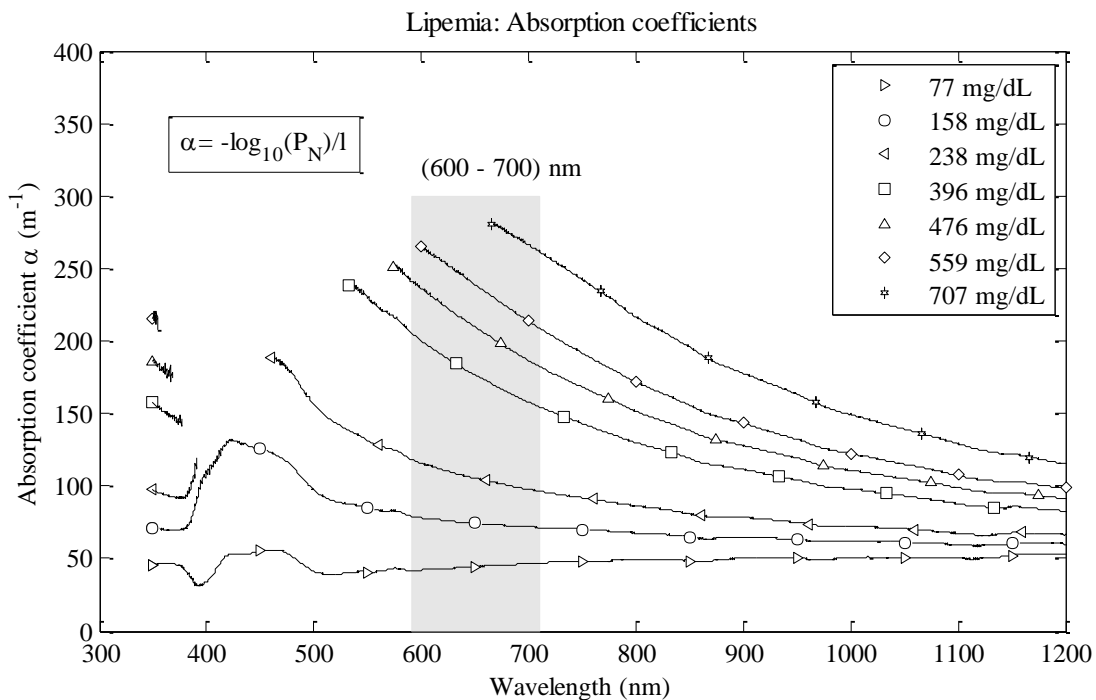
Figure 3.13 Absorption coefficients of Lipemia
