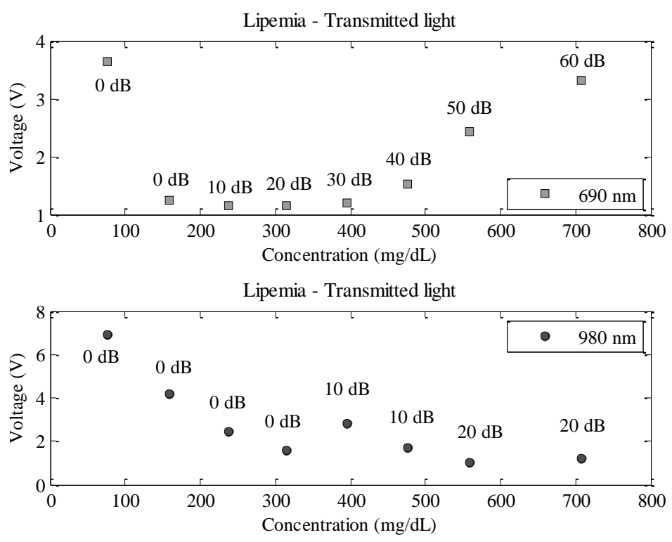
Figure 3.29 Transmitted light for Lipemia as voltage signals at different gain levels
