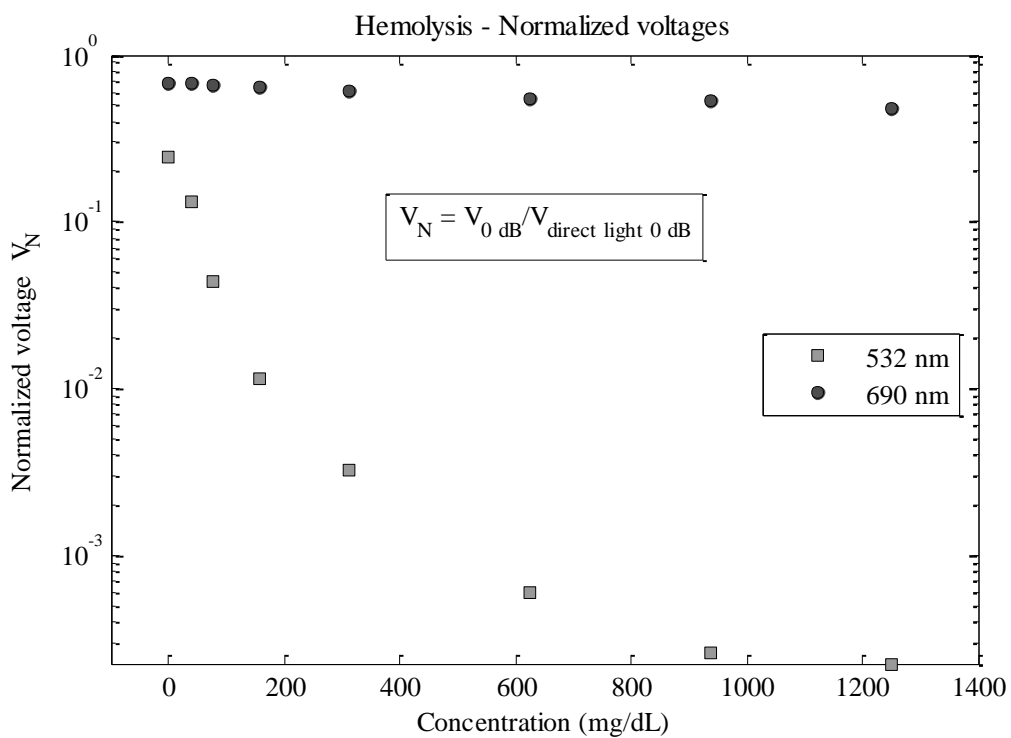
Figure 3.22 Normalized voltage values for Hemolysis
