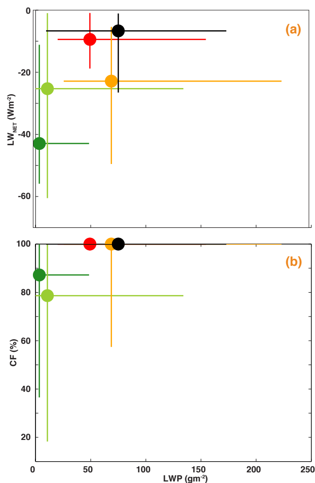
Fig. 8. Figures demonstrating the range of values of liquid water path for observations and models that provide it, as well as its relationship to surface net longwave radiation (a), and cloud fraction (b). The circles represent the mean value over the ASCOS observational period, and the whiskers demonstrate the extent of the 10th and 90th percentiles of the data sets.
