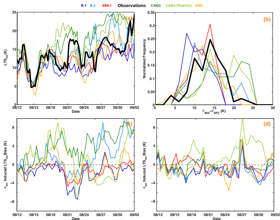
Fig. 10. Time series (a) and histograms (b) of lower tropospheric stability ( LTS_{850} ), as defined by the potential temperature difference between 850 mb and the surface. The lower panels (c, d) illustrate the relative contributions of near-surface potential temperature and the potential temperature at 850 mb to biases in LTS_{850} .
