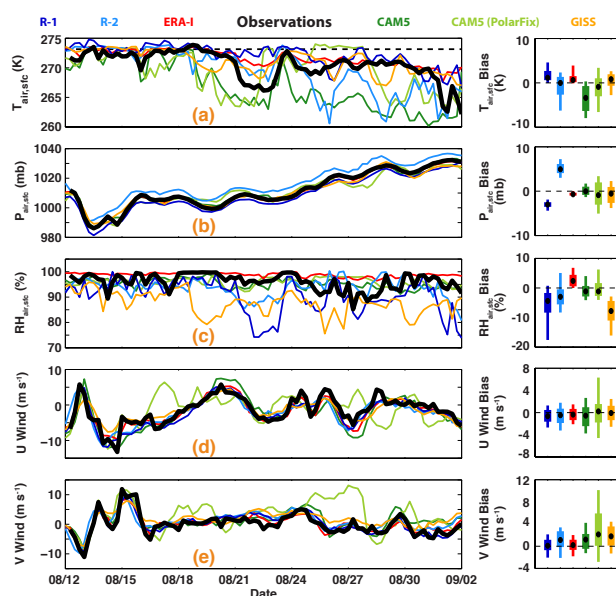
Fig. 2. Time series of basic meteorological quantities from top to bottom: surface air temperature, surface air pressure, surface air relative humidity, 10 m U wind component, and 10 m V wind component. Included are lines for the observations from Oden (bold black line), CAM5 (standard version, dark green; CAM5-PF, light green), the GISS-ModelE2 (orange), and R-1 (dark blue), R-2 (light blue) and ERA-I (red) reanalyses. ERA-I, R-1 and R-2 lines represent 6-hourly analysis (0h) time instantaneous values, while the CAM5 lines depict the interpolated value for the analysis time from the model 1-hourly averages. The right-hand side of the figure includes distributions depicting the median (black dot), IQR (wide bar) and 10th–90th percentiles (thin bar) of the differences between simulated and observed values.
