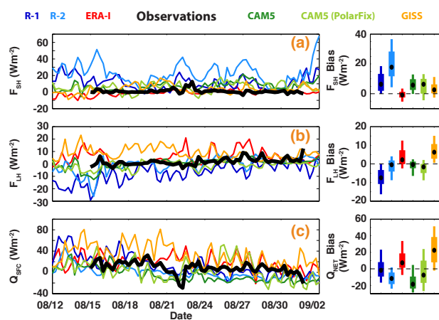
Fig. 6. Time series of surface energy budget terms from top to bottom: average sensible heat flux density, average latent heat flux density, and net surface energy (radiation, latent heat and sensible heat). Included are lines for the observations from Oden (bold black line), CAM5 (standard version, dark green; CAM5-PF, light green), the GISS-ModelE2 (orange), and R-1 (dark blue), R-2 (light blue) and ERA-I (red) reanalyses. All lines represent six-hour average values. The right-hand side of the figure includes distributions depicting the median (black dot), IQR (wide bar) and 10th–90th percentiles (thin bar) of the differences between simulated and observed values.
