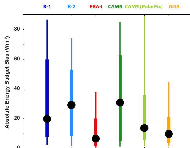
Fig. 7. Combined distributions of the absolute values of biases in LW_{\text{up}} , LW_{\text{down}} , SW_{\text{up}} , SW_{\text{down}} , F_{\text{SH}} and F_{\text{LH}} . Distributions are depicted, including the median (black dot), IQR (wide bar) and 10th–90th percentiles (thin bar).
