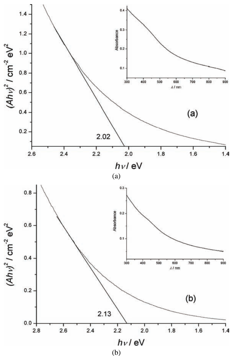
Fig. 3. Plots of (Ah\nu)^2 vs. energy for a) CuInS 2 and b) CuInSe 2 nanoparticles. The insets show the absorption spectrum of the corresponding colloidal dispersions.
