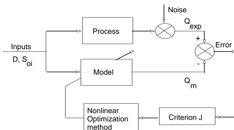
Fig. 1 Non-linear identification method
