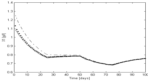
b) Estimates of X_1 , obtained by (10) using R_1 estimates and X_1 estimates by observer (14)
