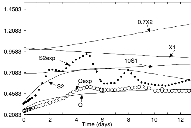
Fig. 2 Evolution of X_1, X_2, S_1, S_2, S_{2exp}, Q and Q_{exp} in the case of one step addition of acetate and S_{0i} = 68 \text{ g}\cdot\text{l}^{-1}
