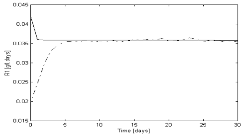
a) R_1 estimates compared with model data
