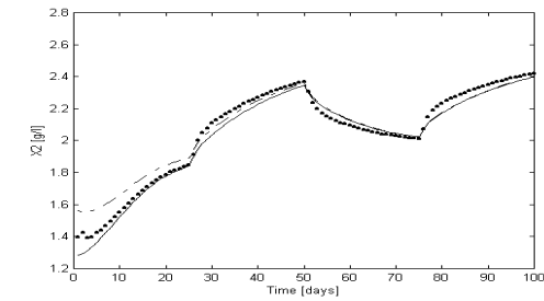
d) Estimates of X_2 , obtained by (20) and (24) respectively
