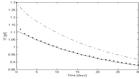
b) Estimates of X_1 , obtained by (10) using R_1 estimates and X_1 estimates by observer (14)
