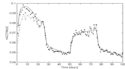
e) Estimates of \mu_2 , obtained by Eq. (22) and (25) respectively
