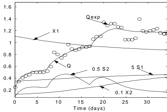
Fig. 3 Evolution of X_1, X_2, S_1, S_2, Q and Q_{exp} in the case of three step additions of acetate and S_{0i} = 7.5 \text{ g}\cdot\text{l}^{-1}
