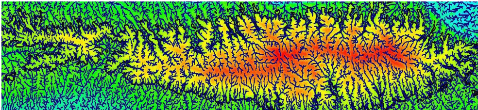
Figure 2. Hypsometry map of Fruska Gora Mountain
