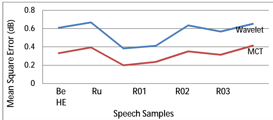
(a) Mean Square Error (MSE)
