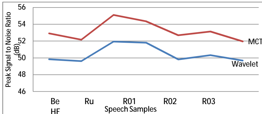
(b) Peak Signal to Noise Ratio (PSNR)
