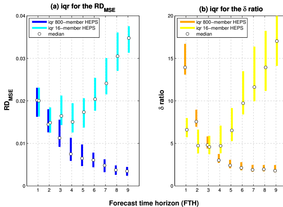
Fig. 3. Interquartile range (iqr) of RD_{MSE} and \delta ratio assessed in the 28 catchments under two HEPS schemes: 16-member HEPS (16 hydrological models are driven by the deterministic forecast from ECMWF) and the 800-member HEPS (16 hydrological models are driven by the 50-perturbed member forecast from ECMWF).
