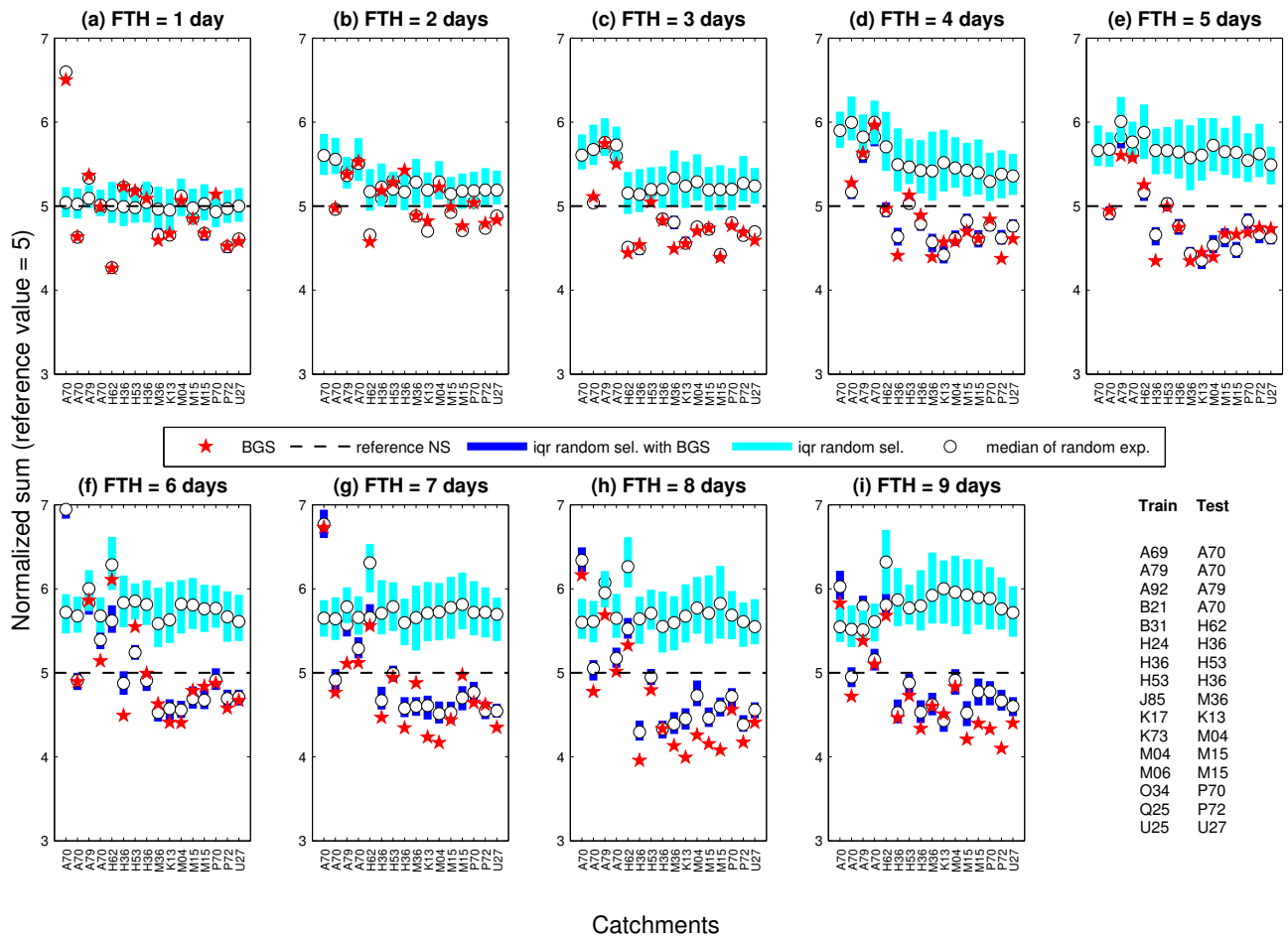
Fig. 6. Evolution of the normalized sum (NS) to evaluate the response sensibility of the extrapolation of results in the nearest catchments. Each vertical bar represents the interquartile range (iqr) of 200 combinations of 50 hydrological members under the following guidelines: the combination is oriented with the same proportion of hydrological models found with BGS-CV (blue vertical bars), the selection is completely random (cyan vertical bars). Note the deficiency of the selections’ extrapolation in basin A69 to basin A79, notably for early lead times (2 to 5 days); these results do not appear in the figure because they are above 7.
