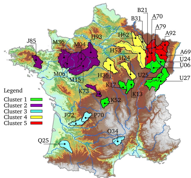
Fig. 1. Location of the catchments grouped by clusters. Some of them have been used in the BGS-CV process, while the others have been used for extrapolation. The colours identify the five regions evaluated in this paper.
