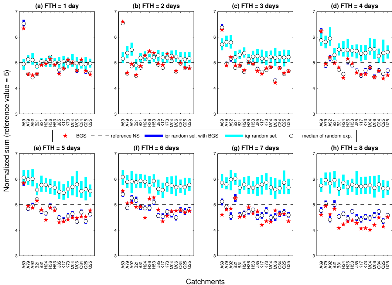
Fig. 4. Evolution of the normalized sum (NS) to evaluate the response sensibility with regard to the interquartile range (iqr) of 200 random experiments in different FTHs following these guidelines: (1) Considering the participation of hydrological models found with BGS-CV (vertical blue bars), and (2) Without regard to any “a priori” participation of hydrological models, i.e. completely random selection (vertical cyan bars).
