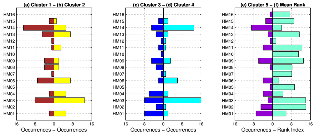
Fig. 7. Hydrological Models participation. Distribution in the five regions (clusters) are presented in (a)–(e). Model performance evaluated as the mean rank index is shown in (f).
