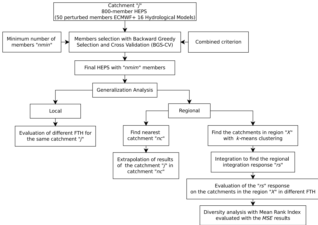
Fig. 2. Generalization test methodology for the hydrological members’ selection found with BGS-CV.
