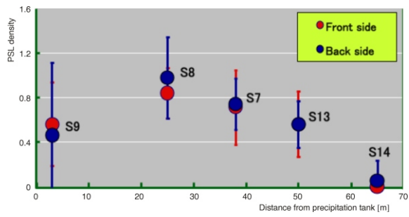
Figure 7. Relation between sampling point and the photo-stimulated luminescence (PSL) density by IP
