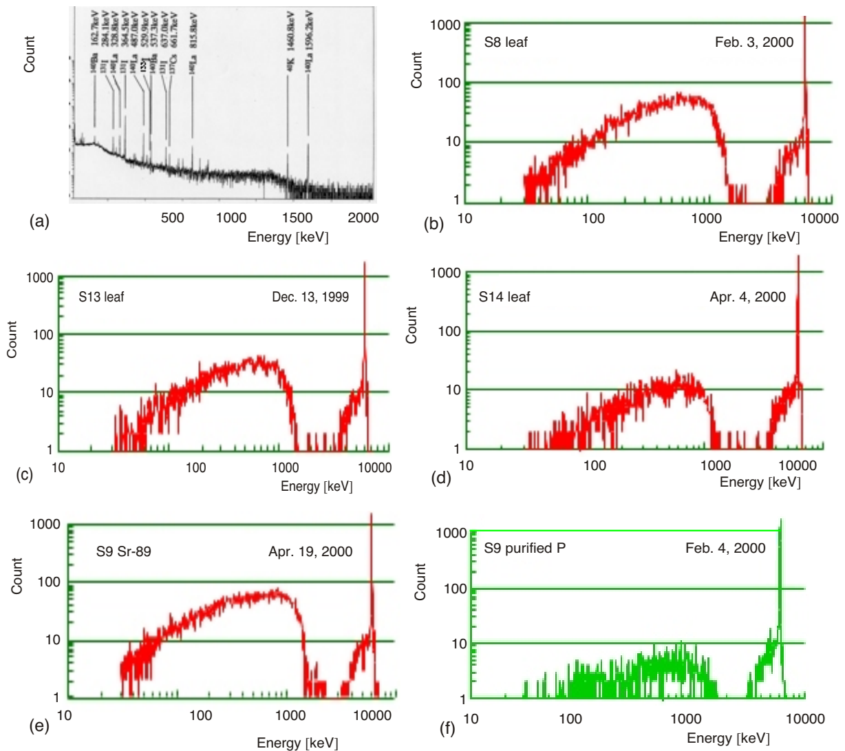
Figure 9. Gamma ray and beta ray spectrum from wormwood collected within the JCO site (a) gamma ray spectrum from wormwood, (b-d) beta ray spectrum from wormwood leaves, (e-f) identification of the beta ray emission nuclide by the beta ray spectrometer after the purification of Sr (e), and of P (f)
