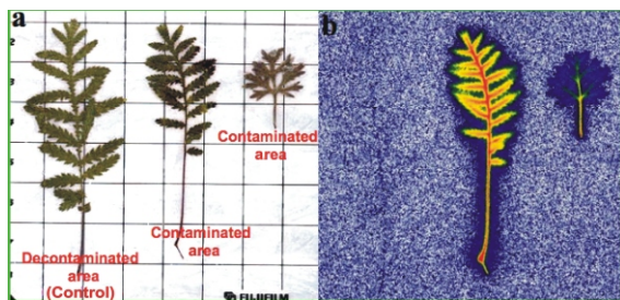
Figure 1. IP analysis of fern leaves (a) photograph of fern before exposure to IP (b) photograph after exposure to IP (exposure time was 24 h)
