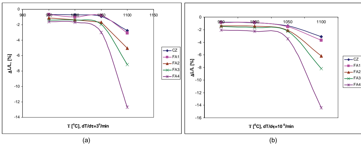
Figure 6. Shrinkage of sintered fly ash compacts using heating rate: a - 3 and b - 10 °C/min.
