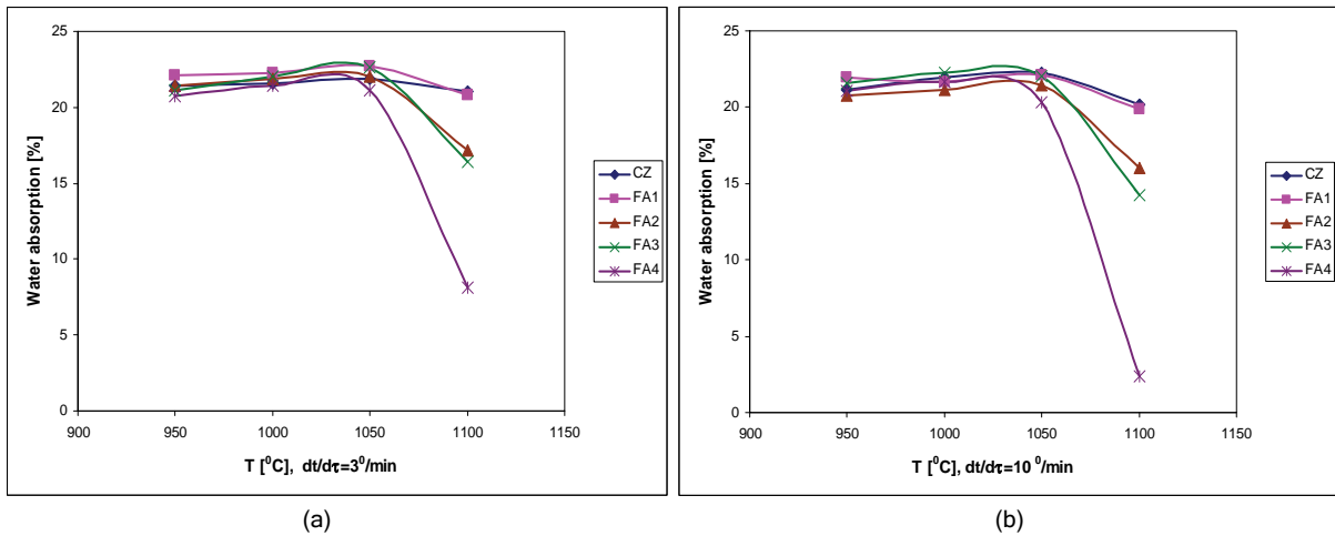
Figure 5. Water absorption of the sintered fly ash compacts using heating rate: a - 3 and b - 10 °C/min.
