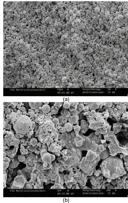
Figure 9. SEM Images for CZ, T = 1100\text{ °C}/1\text{h} , dT/dt = 10\text{ °C}/\text{min} ; bars: a) 10 and b) 2 \mu\text{m} .
