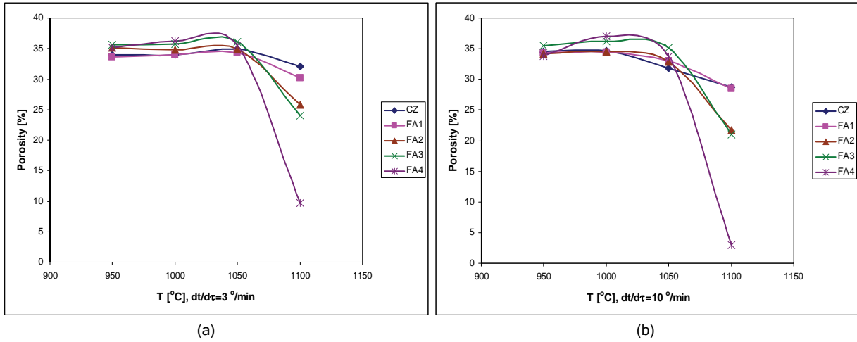
Figure 4. Porosity of the sintered fly ash compacts using heating rate: a - 3 and b - 10 °C/min.
