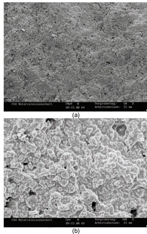
Figure 10. SEM Images for FA4, T = 1100\text{ °C}/1\text{h} , dT/dt = 10\text{ °C}/\text{min} ; bars: a) 10 and b) 2 \mu\text{m} .
