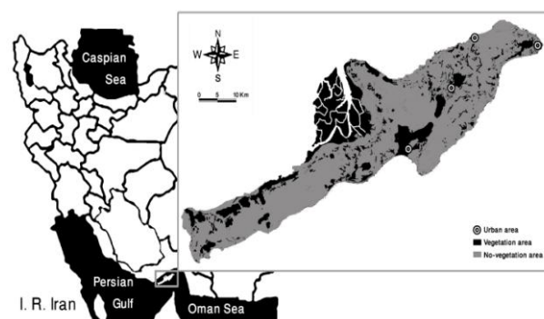
Fig 1. Vegetation area, no vegetation area, and urban area of Qeshm Island, the largest island of the Persian Gulf, southern Iran
