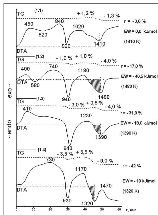
Figure 1 The DTA/TG diagrams for the CuSn5Zn5Pb melting condition with the indicators EW and r (slag composition – Table 2)
