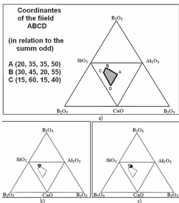
Figure 4 Ranges of optimum concentrations with analysis the graphs of system \text{Al}_2\text{O}_3 - \text{SiO}_2 - \text{CaO} - \text{B}_2\text{O}_3 in basing about measurements: a) of stickiness and melting-point, b) with proposed programme, c) after the DTA investigation
