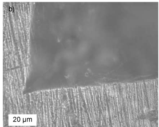
Figure 6. a) Micrograph of the indentation imprint on bone cement after 300 cycles, b) Detail of the indentation imprint on PMMA after 300 cycles (left bottom angle)
