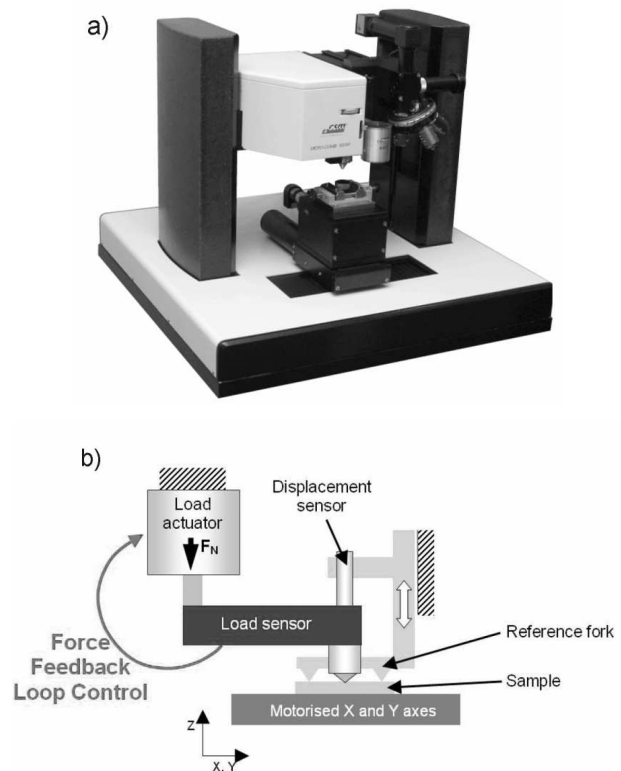
Figure 4. a) CSM Micro Indentation Tester b) Schematic view of the main elements of Micro Indentation Tester
