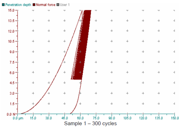
Figure 5. Normal force versus penetration depth curve during micro indentation
