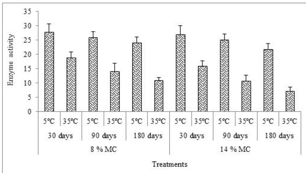
Figure 5. The effect of duration of storage × temperature × moisture contents interaction on catalase activity of sorghum seeds.
