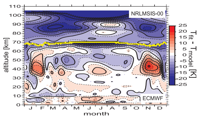
Fig. 9. Difference of fitted lidar observations and reference data sets. Above the yellow line the NRLMSISE-00 is used as reference, below ECMWF-analyses.
