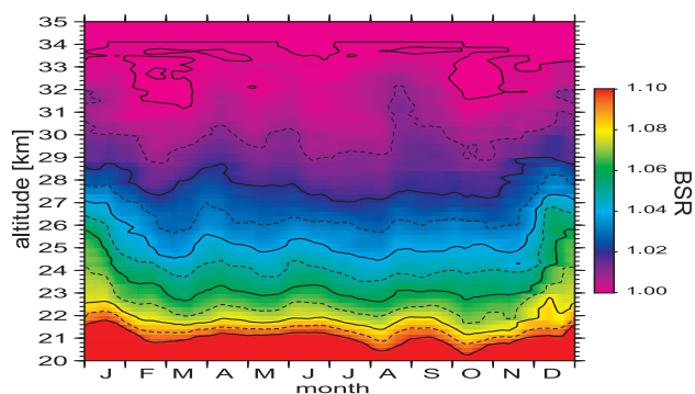
Fig. 2. Seasonal variation of backscatter ratios (BSR) at 532 nm wavelength (213 nights, 11 February 2004–31 July 2007).
