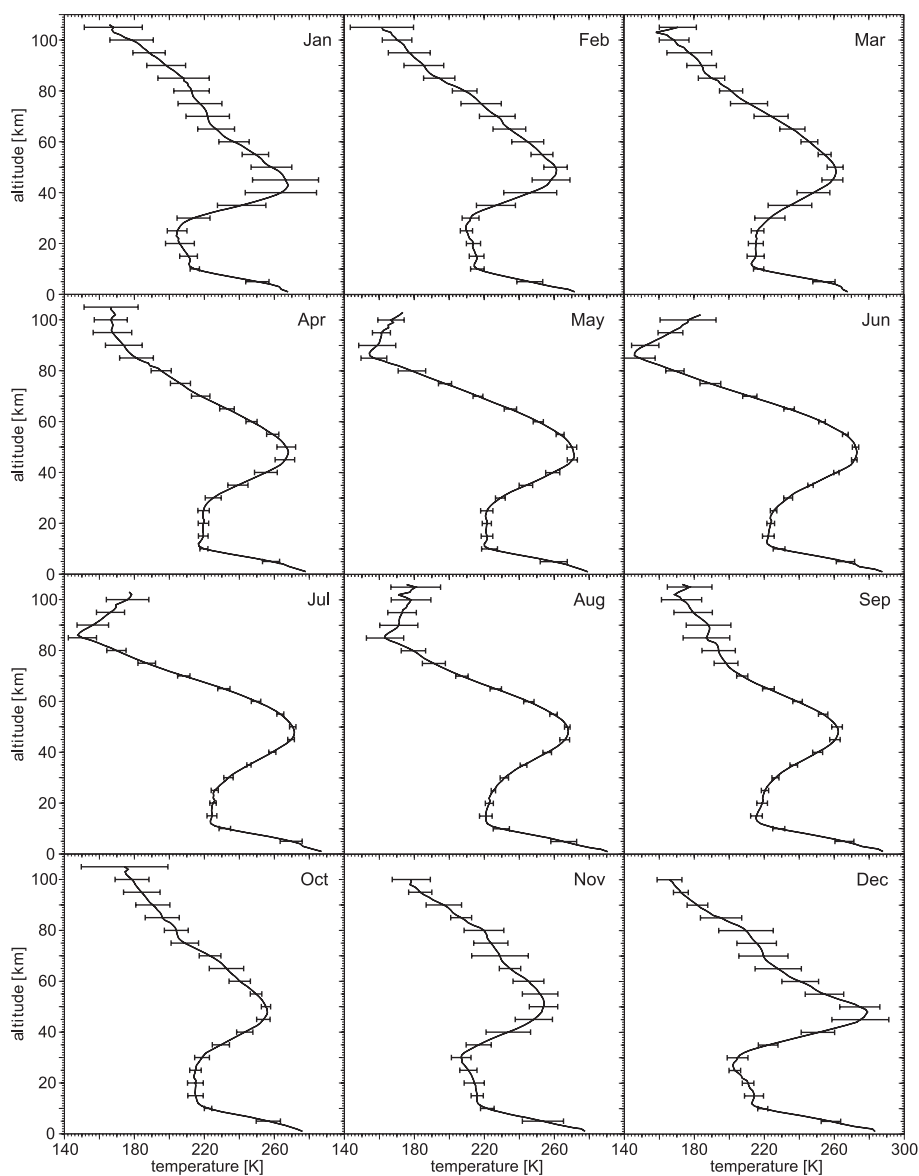
Fig. 4. Monthly averages of nightly mean temperatures between 1 and \sim 110 km altitude. The horizontal bars denote the standard deviations of the nightly mean temperatures (i.e. natural variability but not statistical uncertainties).
