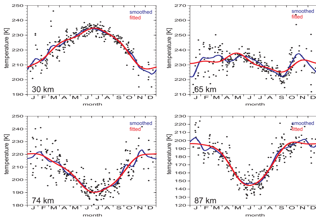
Fig. 5. Seasonal temperature variation at different altitudes. Black dots: nightly mean temperatures, blue line: filtered with \pm 30 day Hanning window, red line: harmonic fit.
