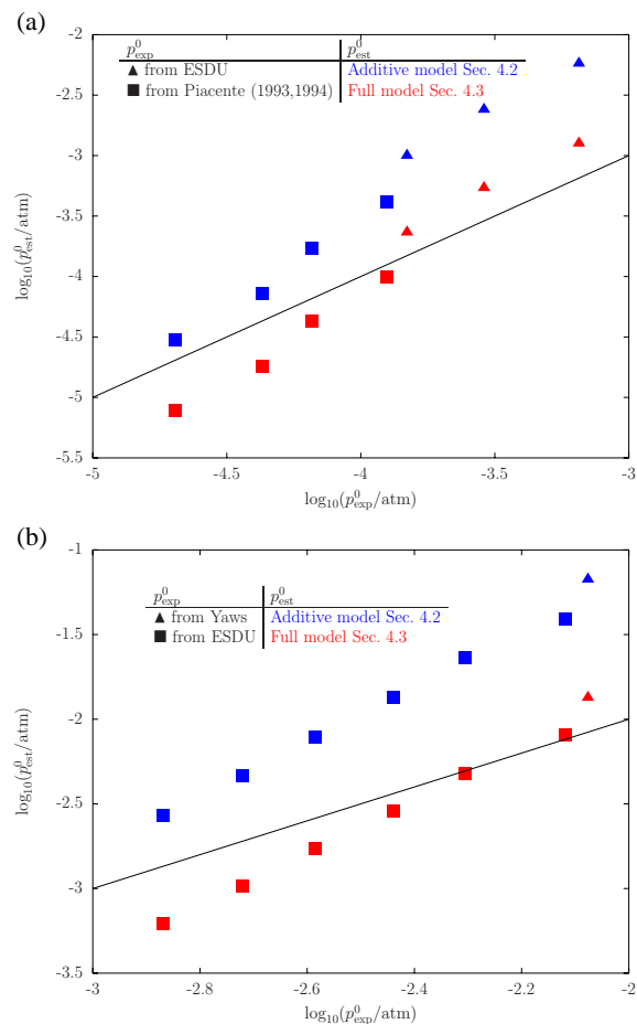
Fig. 3. (a): modeled (est) vs. experimental (exp) \log_{10} p^0 for linear \alpha,\omega -diols at 350 K, from butanediol to decanediol. Blue symbols: modeled results are obtained with the additive model of Sect. 4.2. This model, optimised for hydrocarbons and monofunctional compounds, overestimates the vapour pressure. Red symbols: modeled results are obtained with the full model of Sect. 4.3. (b): idem but for \alpha,\omega -diacids at 460 K. Smaller chains (2–3 carbon atoms) are not shown as local group-group interaction effects would mask the general trend. The black line is the 1:1 line.
