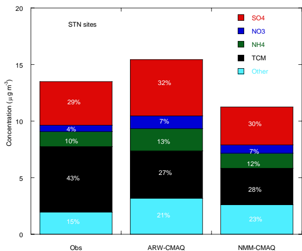
Fig. 4. Comparison of stacked bar-plots for observed and modeled (ARW-CMAQ, NMM-CMAQ) PM 2.5 chemical composition at the STN sites during the 2006 TexAQS/GoMACCS period. The percentages represent the fractions of each composition for PM 2.5 . “OTHER” species refers to unspecified anthropogenic mass which comes from the emission inventory of PM 2.5 .
