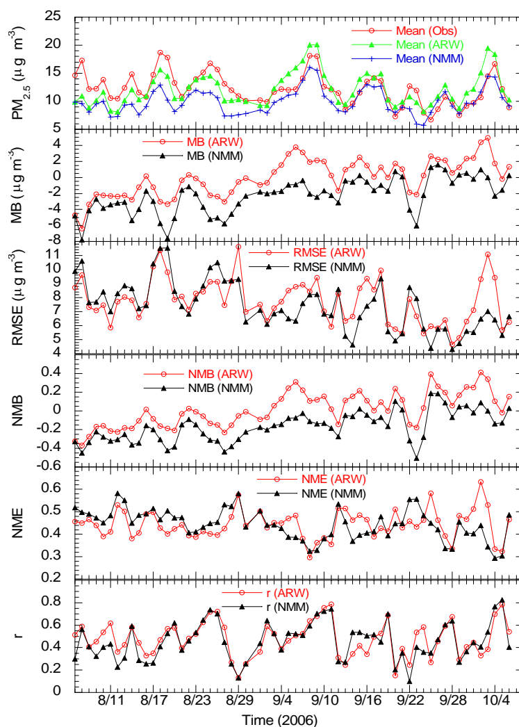
Fig. 2. Comparison of daily variations of the values of domain-wide mean, MB, RMSE, NMB, NME and correlation coefficient ( r ) for the daily \text{PM}_{2.5} mass concentrations at the AIRNow monitoring sites for ARW-CMAQ and NMM-CMAQ simulations.
