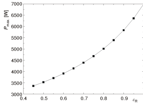
Figure 12. Variation on maximum power output of Stirling engine with respect to regenerator effectiveness
