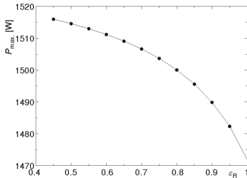
Figure 11. Variation on work output of Stirling engine with respect to regenerator effectiveness
