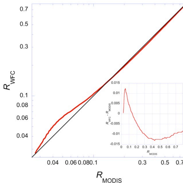
Fig. 2. Comparison of WFC and MODIS 0.65 \mu\text{m} reflectances at the first, second, third, . . . , 99th percentiles of the overall WFC and MODIS reflectance histograms. Inset: difference between WFC and MODIS reflectances at each percentile bin, plotted on a linear scale.
