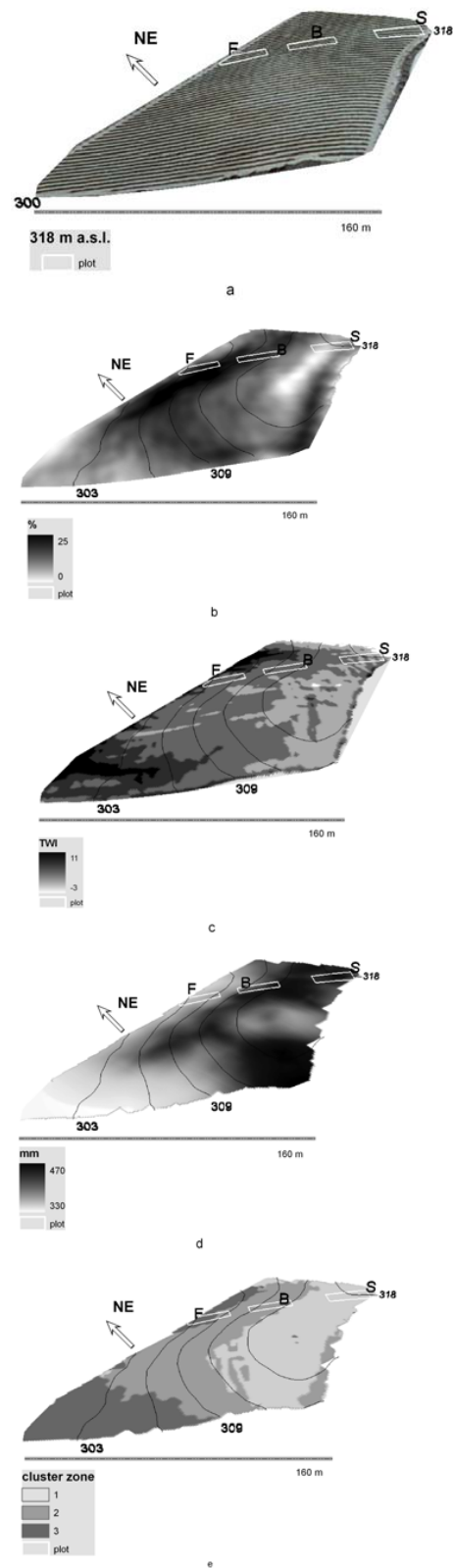
Fig. 2. Vineyard 2; a: 3-D orthophoto with indication of aspect, elevation, and plots (summit S, backslope B, and footslope F); b: slope; c: topographic wetness index (TWI); d: cumulative soil moisture up to the root limiting layer at bud bursting of vines (RL-moist); e: cluster zones.
