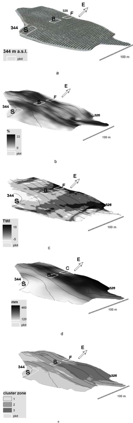
Fig. 1. Vineyard 1; a: 3-D orthophoto with indication of aspect, elevation, and plots (summit S, backslope B, and footslope F); b: slope; c: topographic wetness index (TWI); d: cumulative soil moisture up to the root limiting layer at bud bursting of vines (RL-moist); e: cluster zones.
