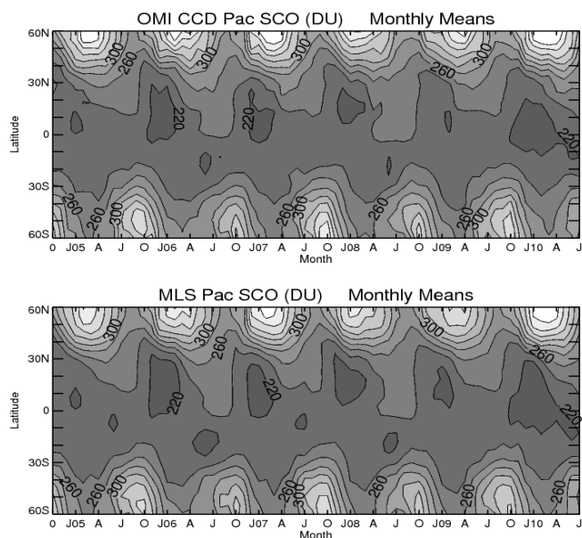
Fig. 8. Latitude versus month contour diagrams of monthly mean stratospheric column ozone (in Dobson Units) averaged over the Pacific (120° W–120° E) from OMI CCD (top) and MLS (bottom). Dark to light shading designates smaller to higher column amounts, respectively. The contour values for both diagrams begin at 200 Dobson units and increment by 20 Dobson Units.
