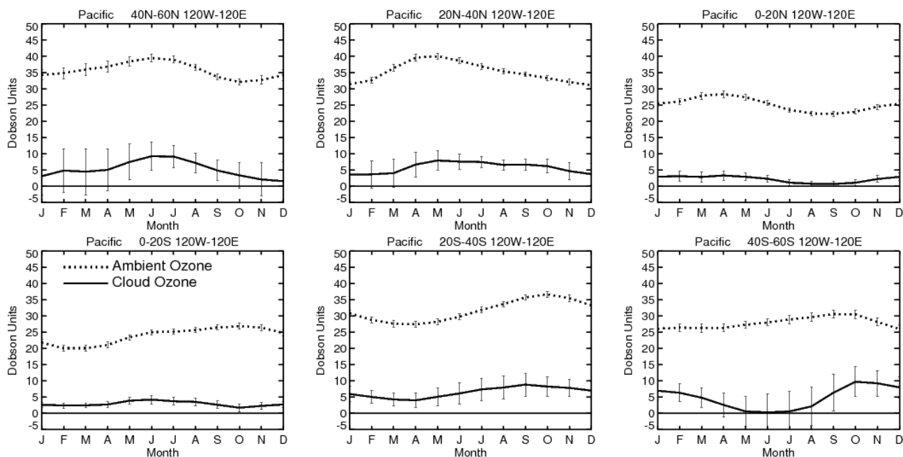
Fig. 5. Solid curves: line plots of CCD 12-month annual cycles of cloud ozone averaged within six non-overlapping 20° latitude bands in the Pacific. The latitude bands are (from upper left to lower right): 40–60° N, 20–40° N, 0–20° N, 0–20° S, 20–40° S, and 40–60° S. The Pacific averaging is for the longitude domain 120° W–120° E about the dateline. Dotted curves: same as solid curves but for background ambient tropospheric column ozone from OMI/MLS residual. These annual cycle time series are all derived by averaging together data for similar months over the six years. The vertical bars represent calculated \pm 1\sigma RMS standard error of mean.
