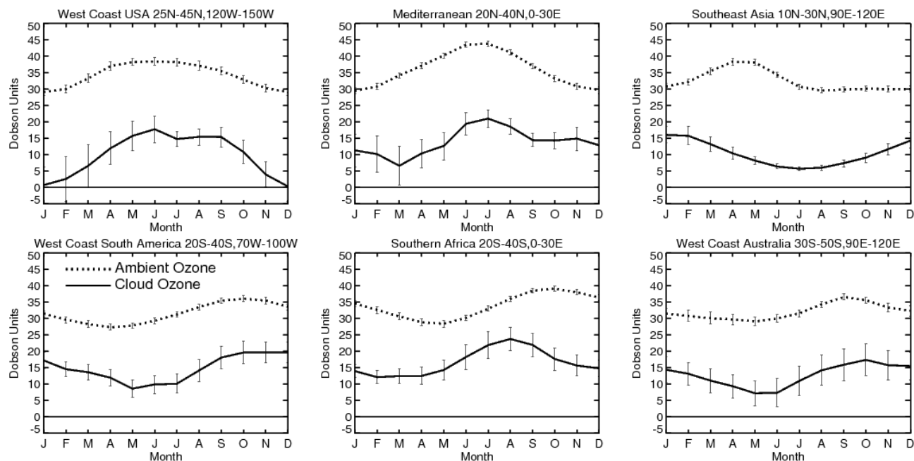
Fig. 7. Similar to Figs. 5 and 6 but instead for six broad regions of the globe where measured CCD cloud ozone is large with peak abundances of \sim 15\text{--}20 DU. These six regions are from upper left to lower right (compare these regions with Fig. 4): West Coast of the USA, Mediterranean, Southeast Asia, West Coast of South America, Southern Africa, and West Coast of Australia.
