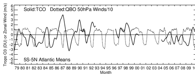
Fig. 14. Tropospheric column ozone from the CCD method in Dobson Units (solid curve) plotted versus 50 hPa zonal winds from Singapore ( 1^\circ\text{N} , 104^\circ\text{E} ) in units \text{m s}^{-1} but divided by 10 for scaling (dotted curve). The ozone time series was averaged over the equatorial Atlantic region ( 5^\circ\text{S}\text{--}5^\circ\text{N} , 60^\circ\text{W}\text{--}60^\circ\text{E} ). The ozone time series was deseasonalized and detrended, and then smoothed using a recursive low-pass digital filter with one-half filter response at 12-month period (filter response of about 0.8–0.9 for 24–36 month QBO time periods).
