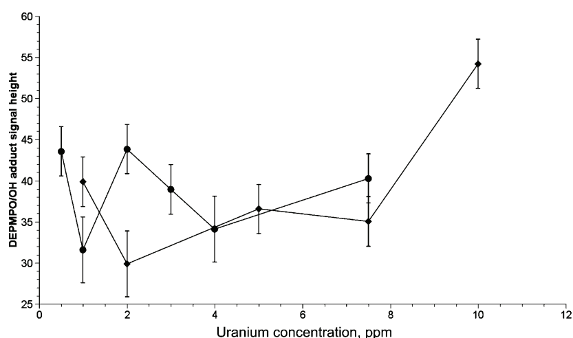
Fig. 5. Uranium concentration dependence of the signal of DEPMPO/OH, produced in solutions of uranyl acetate (●) and uranyl nitrate (◆), pH 2.0, by irradiation with UVB light.
